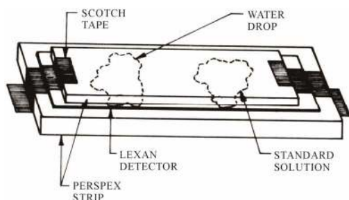
Figure 3. Experimental arrangement of the unknown and known sample assembly for neutron irradiation in the reactor.
