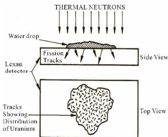
Figure 2. Schematic representation of the neutron induced fission track analysis technique.
