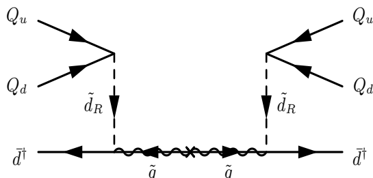
Figure 6. Neutron-Antineutron transitions from R-violating renormalizable operators [98]. Our model does not generate this diagram, but the alternative one in figure 3.
