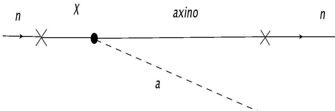
Figure 9. Example of a mechanism for UHECR protons propagation, involving rapid oscillations between neutron and neutralino \tau_{n-\chi} \simeq 1-500 s; neutralino decay into axion and axino with \tau_{\chi \rightarrow a\tilde{a}} > (5 \div 10)\tau_{n-\chi} and finally the transition of the axino into the neutron with \tau_{\tilde{a}-n} \gg \tau_{n-\chi} .
