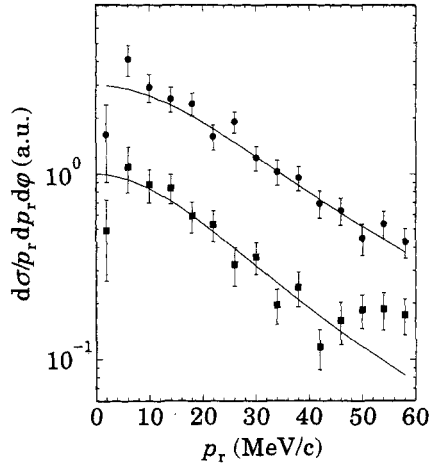
Fig. 3. – As fig. 2 but for ^{11}\text{Be} reacting on a C at 460 MeV/u. Filled circles denote the distributions in coincidence with ^7\text{Li} and filled squares the ones in coincidence with ^8\text{Li} .
