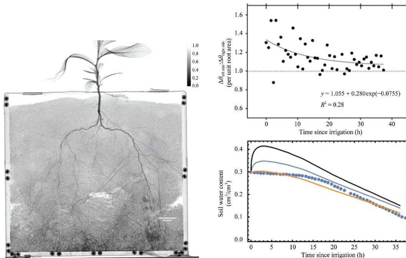
Figure 16 Left: 11-week-old poplar seedling in sand. The intensity indicates the water content. Greater initial water uptake per unit root area is observed for the left side (of the chamber), which has younger, finer diameter roots. Right: water content based on measured NR (circles) or forward modeling using measured (black) or alternate (blue, orange) soil saturated hydraulic conductivities (Dhiman et al. , 2018). In these studies, nR links root water uptake to characteristic root traits and can assess the performance of common water-uptake models.
