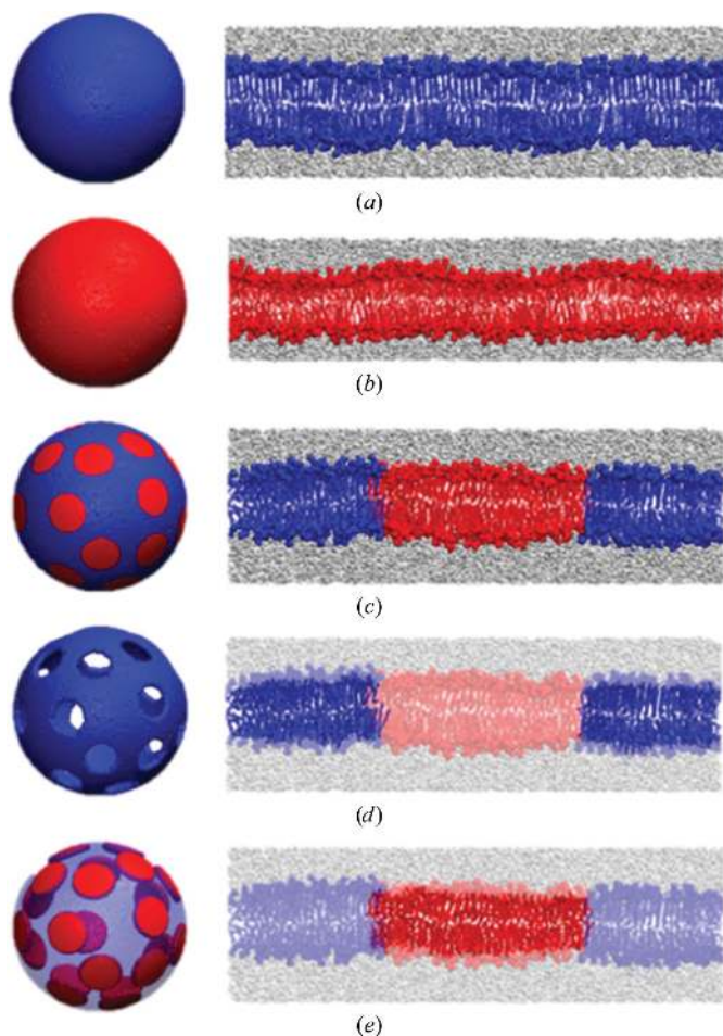
Figure 13 Difference contrast-matched ULVs. (a) L_O ULV. (b) L_D ULV. (c) L_O ULV with L_D nanodomains. (d) L_O ULV with contrast-matched L_D nanodomains. (e) L_D nanodomains with contrast-matched L_D surrounding (Nickels et al. , 2015)
