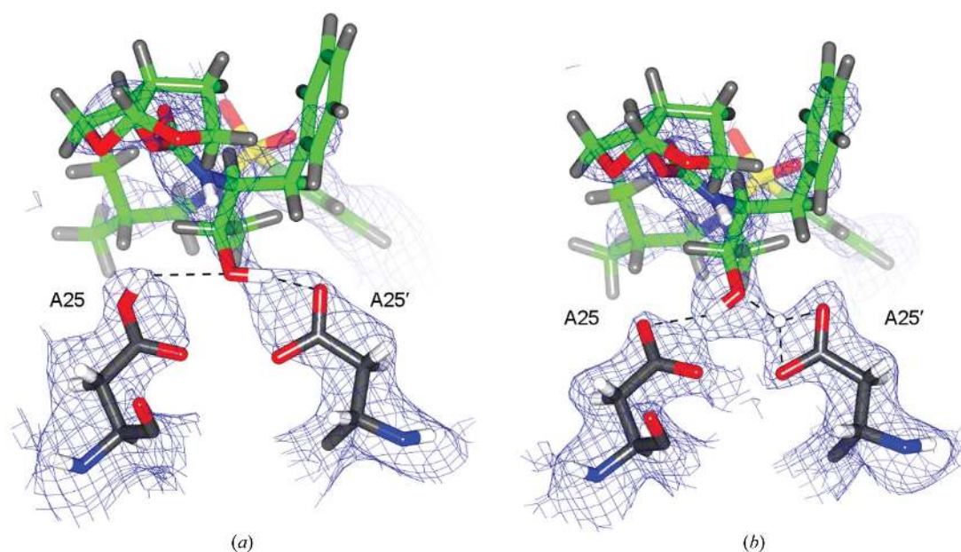
Figure 3 HIV-1 protease in complex with the clinical drug darunavir (PDB entries 5e5j and 5e5k; Gerlits et al. , 2016). Upon homodimerization, the catalytic site contains two closely positioned aspartic acid residues. (a) At pH 4.3, darunavir accepts a hydrogen bond from Ala25 and donates a hydrogen bond to Ala25'. (b) At pH 6.0, the two hydrogens undergo a transfer reaction in the catalytic site, which was captured for the first time by neutron crystallography. C atoms belonging to darunavir are colored green. ^1\text{H} atoms are shown in light gray, while atoms that have undergone exchange to ^3\text{H} are shown in white. The blue mesh represents neutron SLD 2F_o - F_c maps contoured at \sigma = 1.0 . Reproduced from Schröder et al. (2018).
