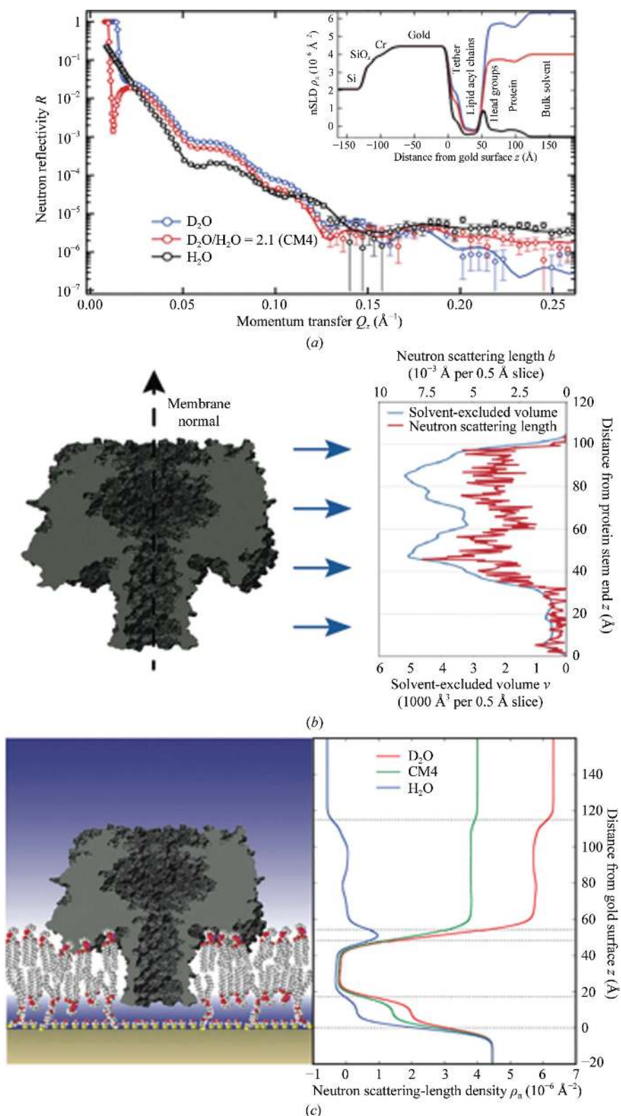
Figure 11 Determination of membrane-protein structures using NR. (a) Proteins embedded in a substrate-supported, in-plane fluid bilayer (lower left) are measured at various solvent contrasts. (b) Integrative modeling uses diverse sources of information, such as protein crystal structures, to model the NR data using rigid-body placement algorithms that determine the penetration depth and orientation of the protein in the membrane. (c) The final model that represents experimental data from NR at different contrasts, crystallographic, volumetric and chemical connectivity information, and thus describes the atomistic protein structure in the supported bilayer.
