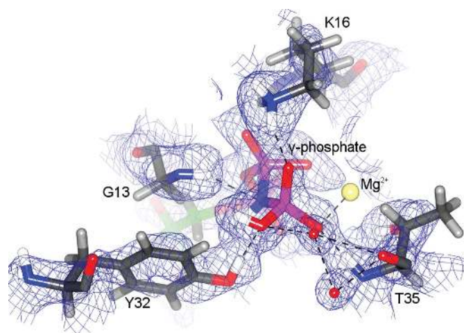
Figure 2 H-Ras in complex with the GTP analog GppNHp (PDB entry 4rsg; Knihtila et al. , 2015). Unexpectedly, clear neutron scattering-length density could be observed for a protonated ( ^2\text{H} ) \gamma -phosphate in the 2F_o - F_c map. The D atoms of the nucleophilic water (hydrogen-bonded to the \gamma -phosphate and Thr35) are not visible in the density map, suggesting rotational freedom. Ligand C atoms are shown in green. ^1\text{H} atoms are shown in light gray, while atoms that have undergone exchange to ^2\text{H} are shown in white. The blue mesh represents a neutron SLD 2F_o - F_c map contoured at \sigma = 1.0 . Reproduced from Schröder et al. (2018).
