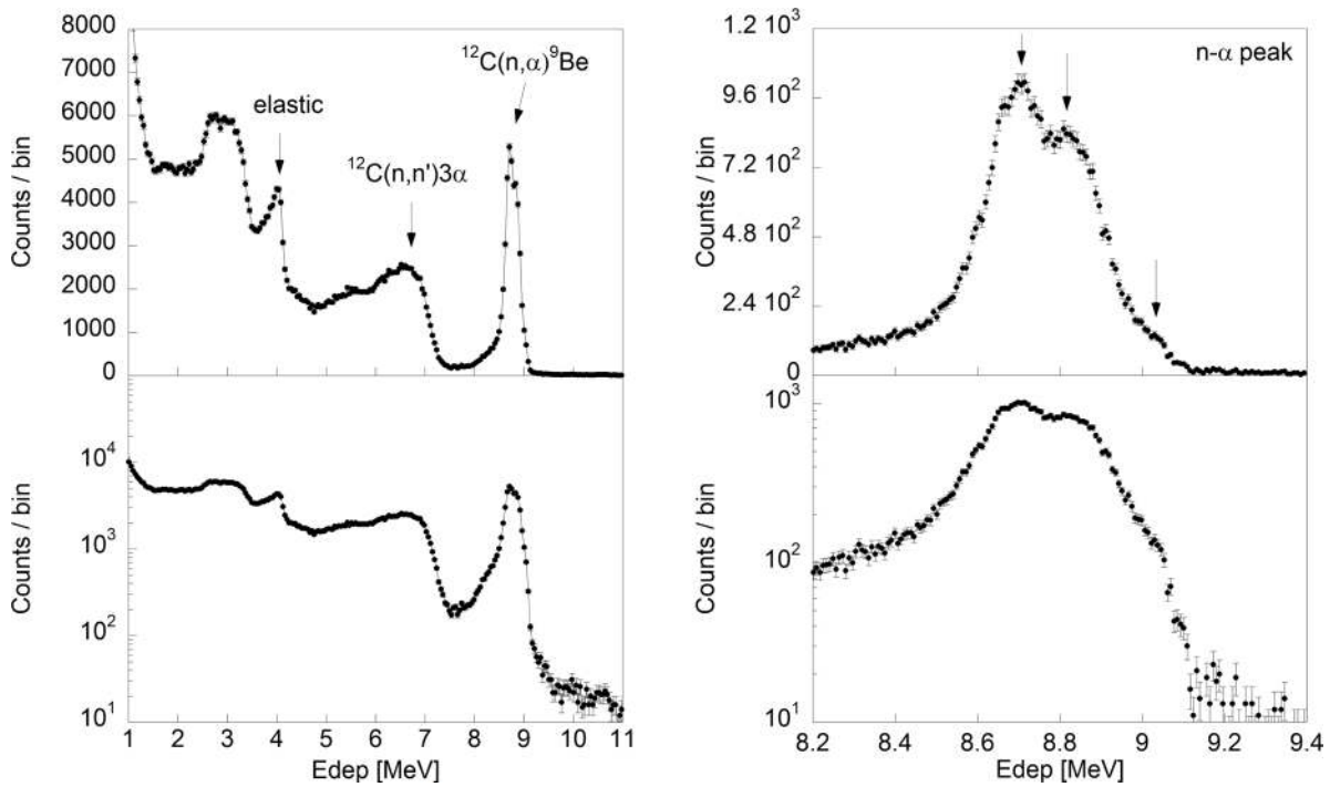
Figure 5. PHS recorded at zero degrees in linear scale (top-left) and logarithmic scale (bottom-left). The n-\alpha peak is shown in detail in linear scale (top-right) and in logarithm scale (bottom-right). The arrows in the plot indicate the main structures in the PHS spectrum and the structures of the peak. E_{\text{peak}} = E_n - 5.702 \text{ MeV} .
