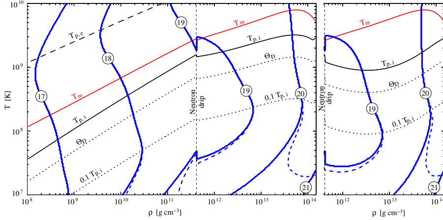
Fig. 4 Iso-contour lines of the electron thermal conductivity \kappa_e in the crust, labeled by the value of \log_{10}(\kappa_e/\text{erg s}^{-1}\text{cm}^{-1}\text{K}^{-1}) , using the results of Gnedin et al. (2001). Also shown are the melting curve T_m , the electron and ion plasma temperatures, T_{p,e} and T_p respectively, the Debye temperature, \Theta_D \simeq 0.45T_p , that marks the transition from classical to quantum solid and 0.1T_p below which the wholly quantum crystal regime is realized. The crust composition is the same as in Fig. 2. The right panel only displays the inner crust but assuming that about 80% of the dripped neutrons are entrained: the strong reduction of T_p and \Theta_D pushes the onset of the wholly quantum regime to lower T . The dashed contour lines illustrate the reduction of \kappa_e from impurity scattering, assuming an impurity parameter Q_{\text{imp}} = 1 .
