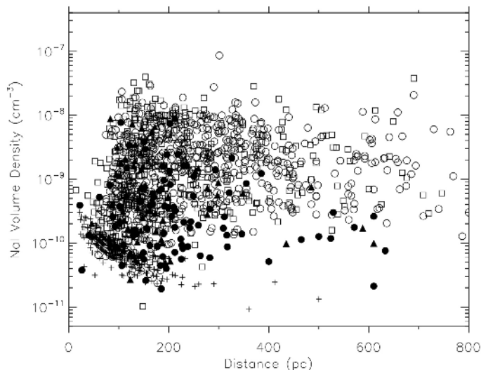
Fig. 9. Plot of the volume density of interstellar NaI absorption for stars with distances <800 pc. Symbols are the same as Fig. 7.
