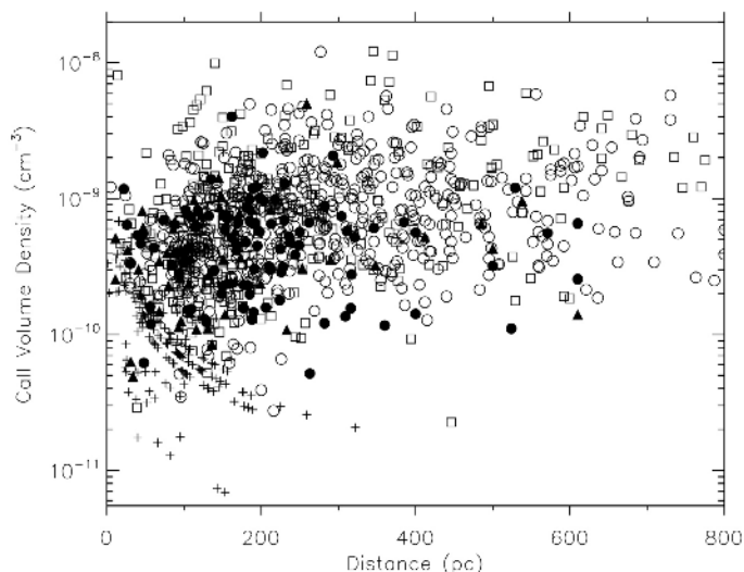
Fig. 10. Plot of the volume density of interstellar CaII absorption for stars with distances <800 pc. Symbols are the same as those in Fig. 7.
