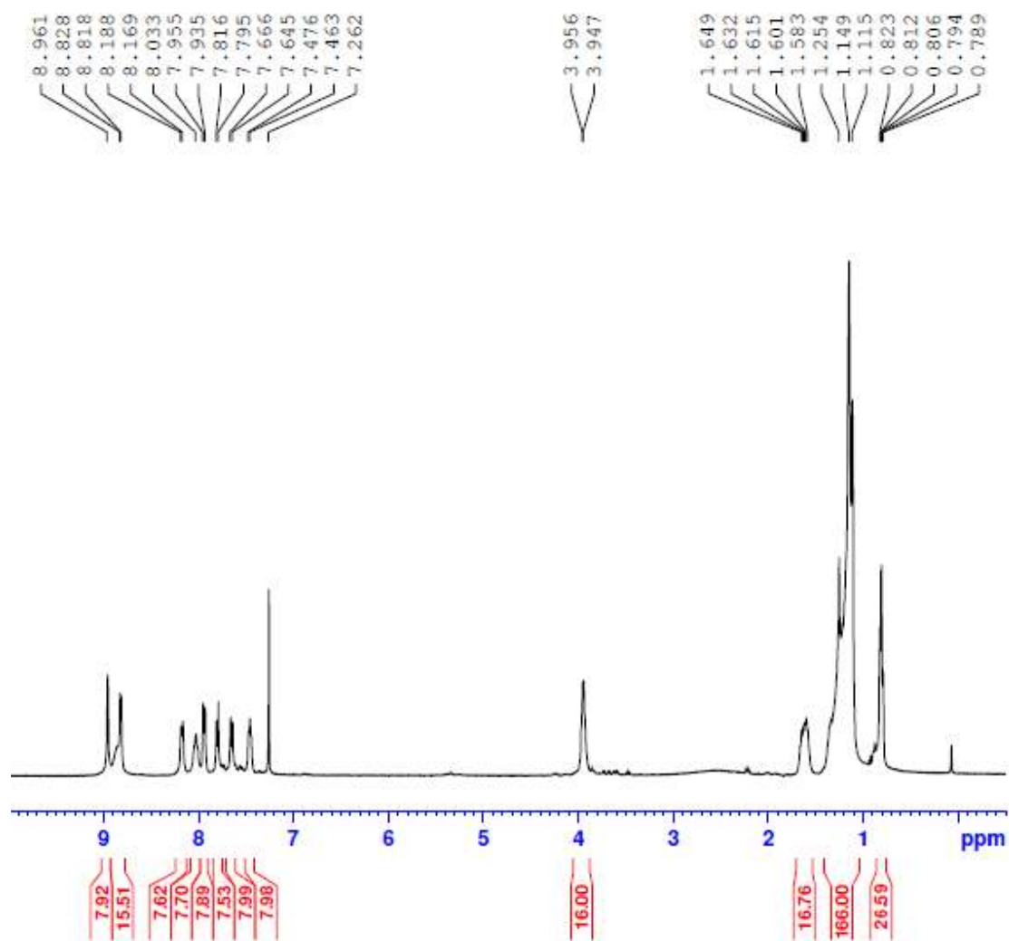
Figure A14 ^1\text{H} NMR spectrum of 1
