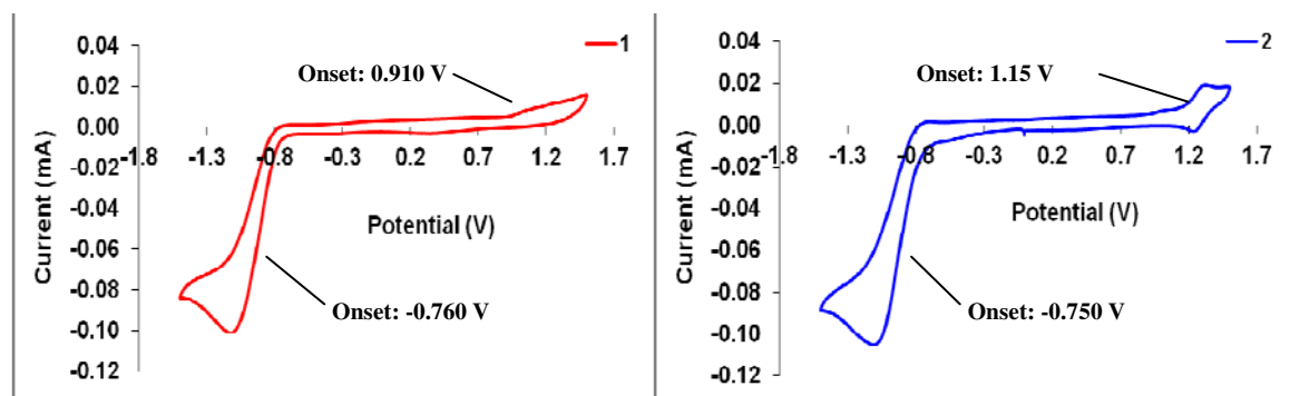
Figure A33 Cyclic voltammograms of 1 and 2 on a platinum electrode (wire) in 0.100 M Bu 4 NPF 6 , DCM solution with a sweep rate of 100 mV/s
