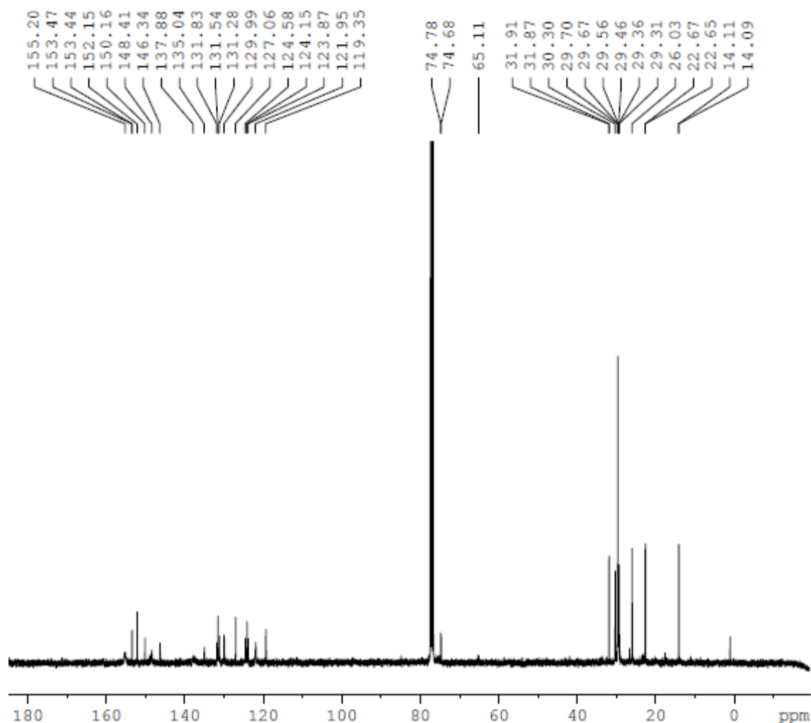
Figure A15 ^{13}\text{C} NMR spectrum of 1
