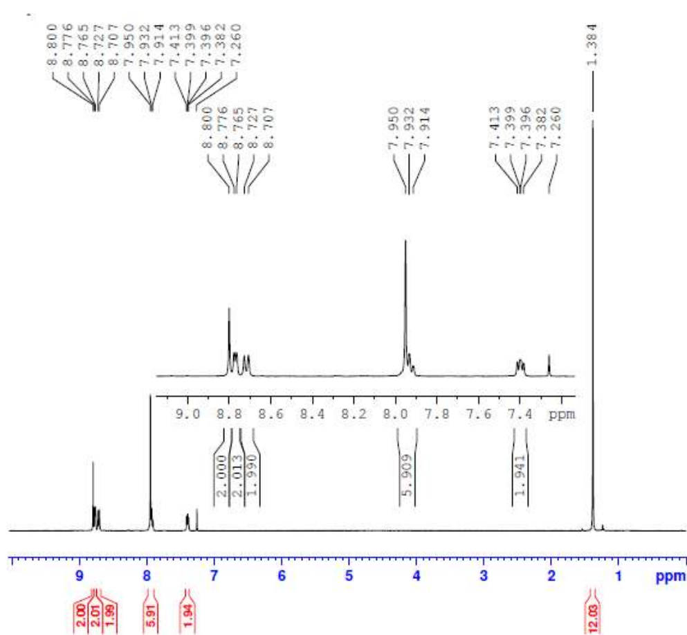
Figure A5 ^1\text{H} NMR of 4'-(4-Pinacolotoboronphenyl)-2,2':6',2''-terpyridine ( 6 )
