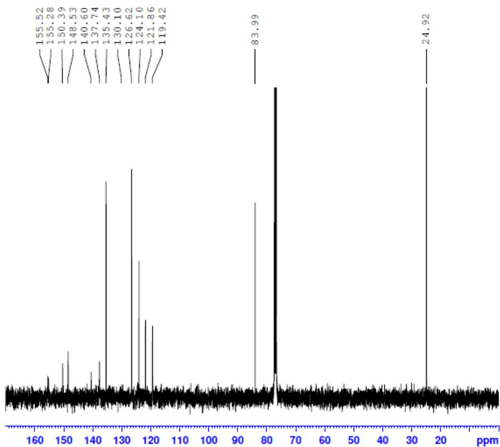
Figure A6 ^{13}\text{C} NMR of 4'-(4-Pinacoloboronphenyl)-2,2':6',2''-terpyridine ( 6 )
