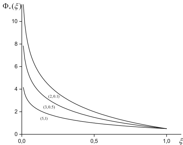
Fig. 5 Typical profiles of the envelope function \Phi_*(\xi) , the solutions to the key equation (48), for the case M^2 > Q^2 and \Phi(1) = 0.5 ; the numbers in parentheses correspond to the values of the parameters \frac{M^2}{Q^2} - 1 and \frac{\mu^2}{\Psi_0^2 M^2} , respectively
