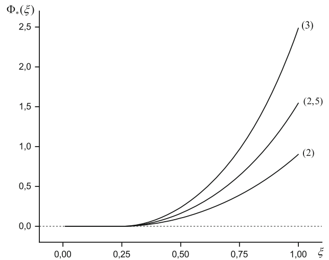
Fig. 3 Illustrations of the stepwise equilibrium function (71) with the envelope function (72). For all profiles \frac{Q_*}{n_*\mu} = 1 and the delimiter is \xi_* = 0.25 . The values of the parameter \Gamma = \frac{\mu}{\Psi_0 M} are written in parentheses
