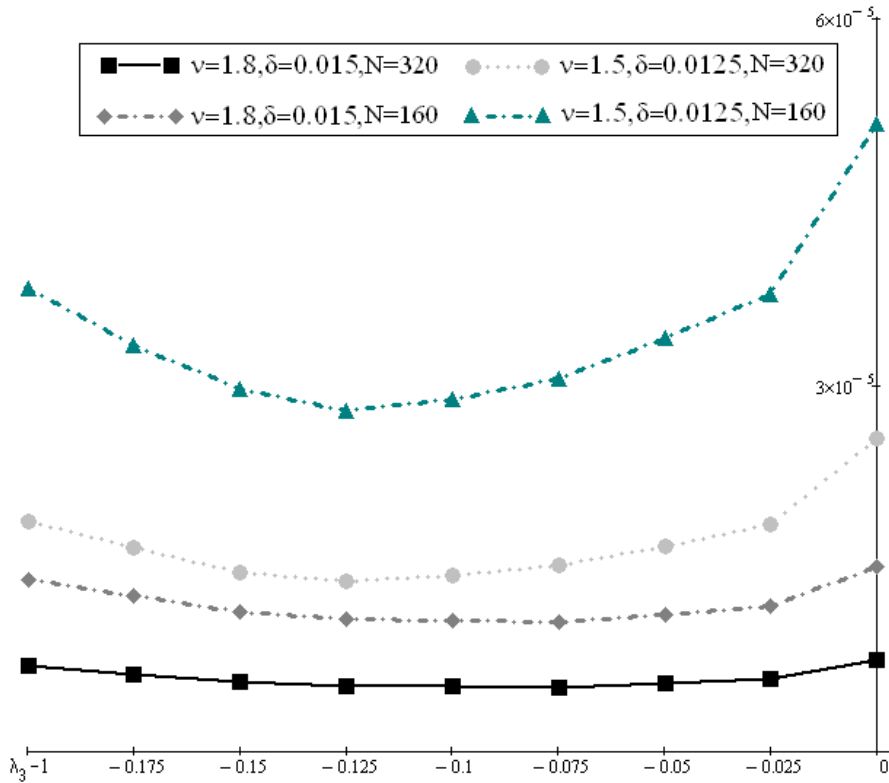
Fig. 5. The dependence of \|\mathbf{u}_\nu^h - \mathbf{u}\|_{\mathbf{W}_{2,\nu}^1(\Omega)} on the degree of \nu^* , for \omega_3 = \frac{9\pi}{8}
