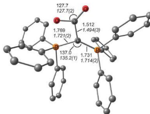
Fig. 3 Calculated (BP86/SVP) and (in italics ) experimental bond lengths and angles of O_2C-C(PPh_3)_2 . 18,31
