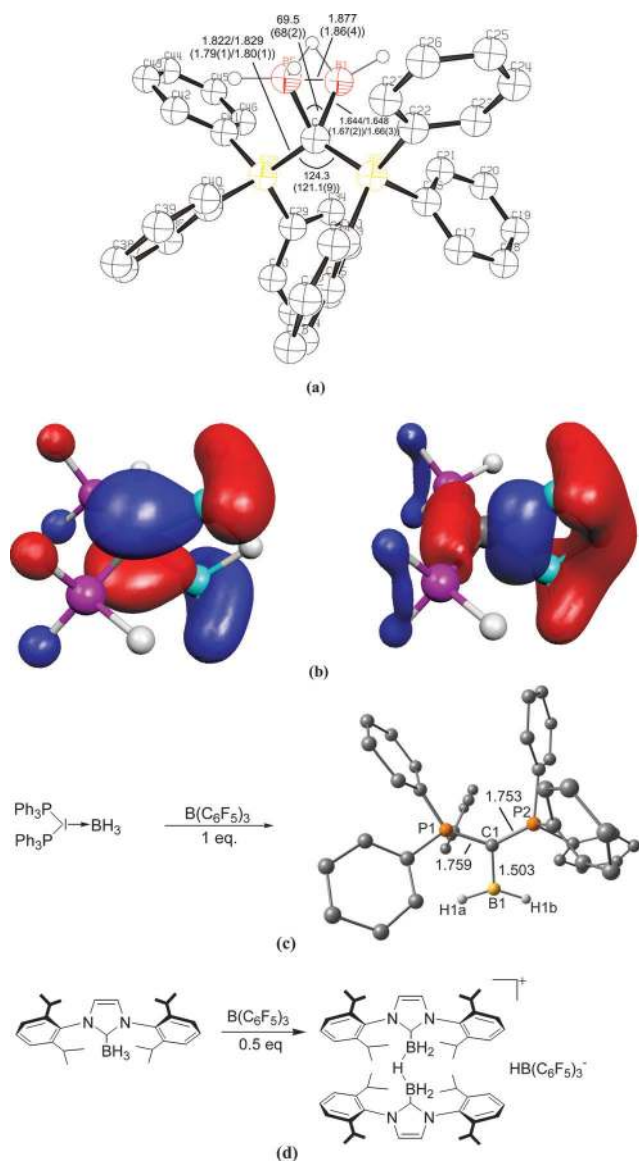
Fig. 4 (a) Calculated at BP86/SVP and (in parentheses) experimental bond lengths and angles of [(\mu-H)H_4B_2]C(PPh_3)_2^+ . 20 (b) Plot of the HOMO and HOMO-1 of [(\mu-H)H_4B_2]C(PPh_3)_2^+ . (c) Reaction of (H_3B) \leftarrow C(PPh_3)_2 with B(C_6F_5)_3 yielding the complex [(H_2B) \leftarrow C(PPh_3)_2]^+ . (d) Reaction of (H_3B) \leftarrow NHC with B(C_6F_5)_3 yielding the bridged complex [NHC \rightarrow \{(\mu-H)H_4B_2\} \leftarrow NHC]^+ . 21
