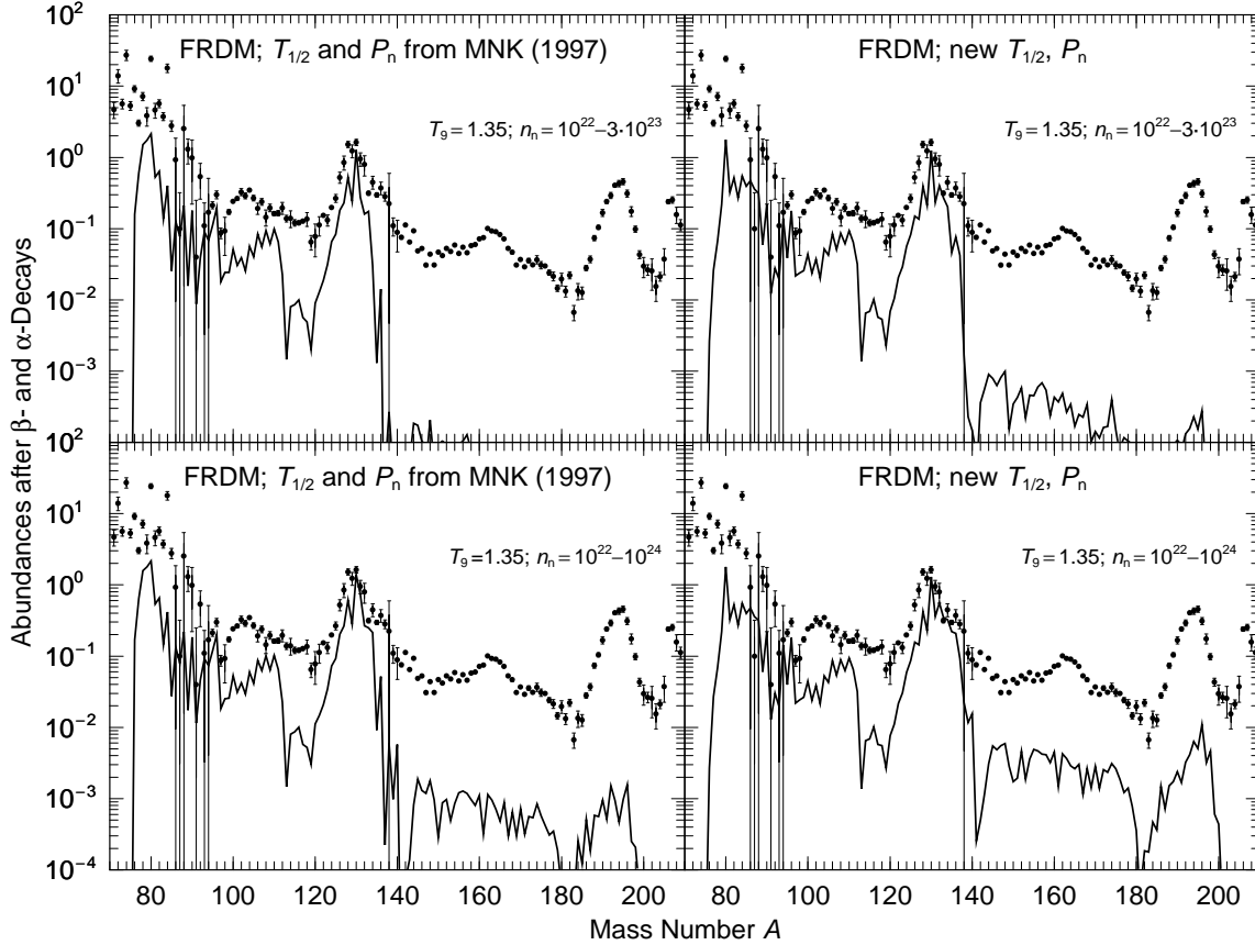
Figure 11: Comparison of calculated r-abundance n_n\text{-}\tau_r components which mainly build the A \simeq 130 N_{r,\odot} peak at a freeze-out temperature of T_9 = 1.35 , using exclusively theoretical T_{1/2}(\text{GT}) and P_n(\text{GT}) values from Ref. [7] (left part) with our new T_{1/2}(\text{GT}+ff) and P_n(\text{GT}+ff) predictions (right part). In all calculations, nuclear masses were used from the Audi evaluation [33] or from the FRDM model [4]. It is clearly evident from this comparison, that – within the same process times \tau_r = 2.00 s for the upper figures and \tau_r = 2.15 s – the shorter T_{1/2}(\text{GT}+ff) result in a faster r-matter flow at the N = 82 bottle-neck region, thus producing already considerably higher r-abundances of rare-earth elements than with the use of the older T_{1/2}(\text{GT}) values. For more details, see text.
