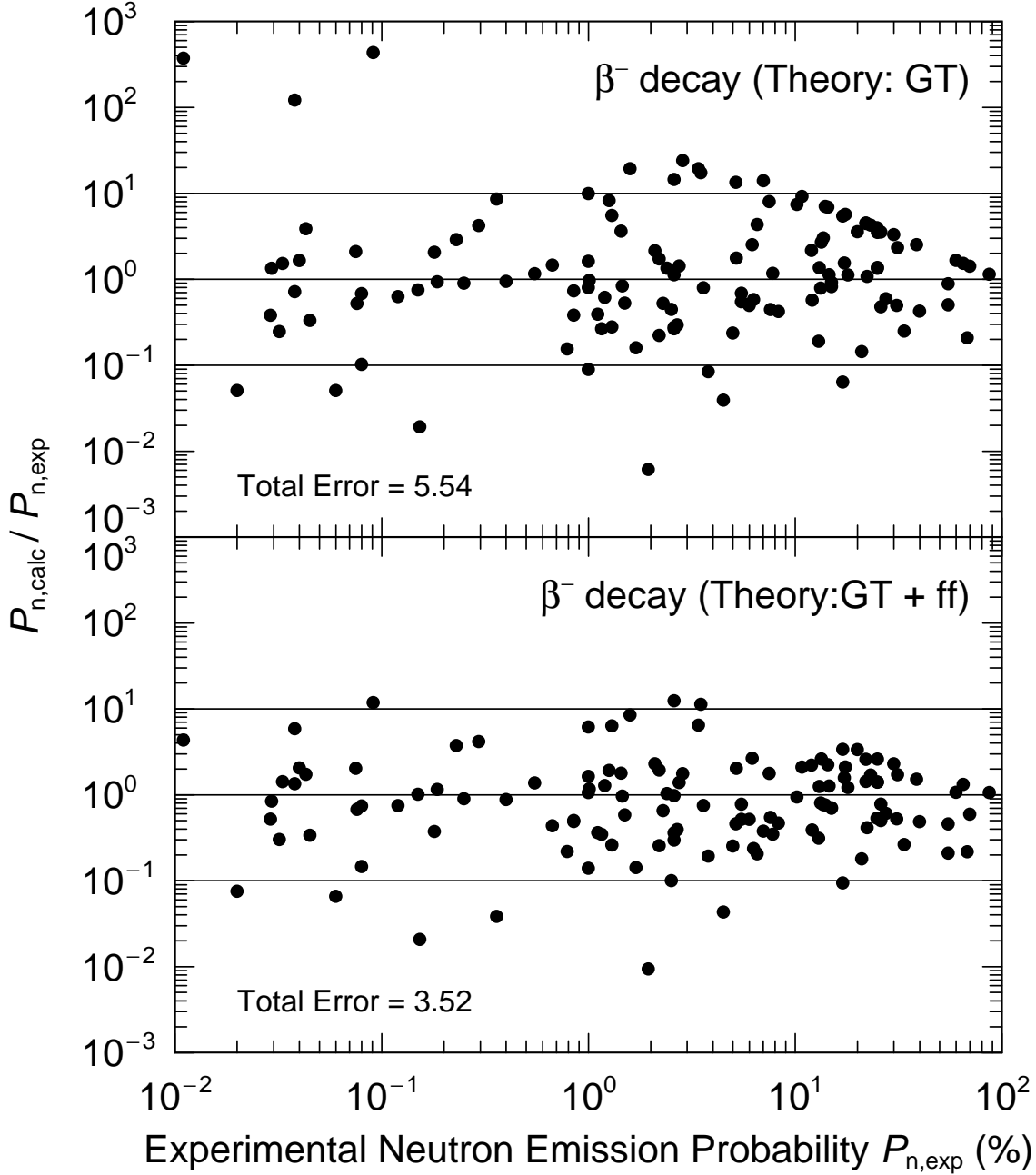
Figure 5: Ratio of calculated to experimental \beta -delayed neutron-emission probabilities P_n for nuclei in the fission-fragment region in our previous and current models.
