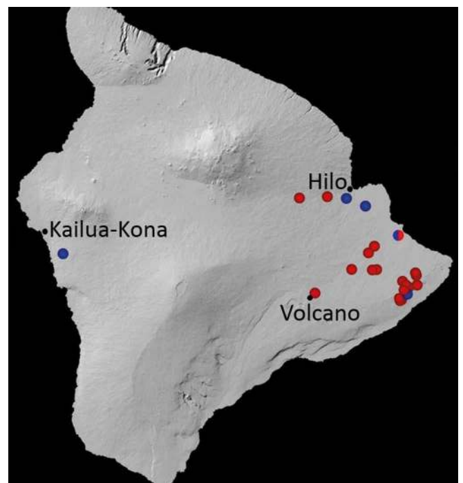
Fig. 1 Distribution of samples yielding isolates of Ceratocystis lukuohia (red circles) and C. huliohia (blue circles) on Hawaiʻi Island during 2014–2015.
