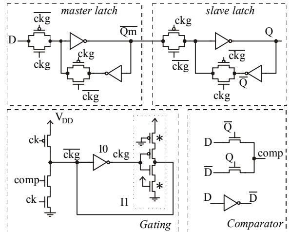
Figure 6. NC^2MOS flip-flop using pass-transistor logic for the comparator. Gating logic transistors sizing is the same of Figure 5 and the NMOS driven by comp has W/L = 3.6\mu m/0.8\mu m . Comparator PMOS and NMOS sizing is W/L = 7.2\mu m/0.8\mu m and W/L = 3.6\mu m/0.8\mu m , respectively.
