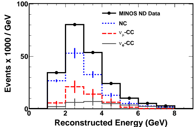
FIG. 1: Reconstructed Near Detector energy spectra of the \nu_e -CC selected events (bold solid). Also shown is the decomposition of this spectrum into neutral current (dotted), \nu_\mu charged current (dashed), and beam \nu_e -CC (light solid) components determined using the multiple beam configuration method. The sum of the three background components is constrained to agree with the data. Uncertainties on the data are statistical and are not visible on this scale; uncertainties on the components are systematic.
