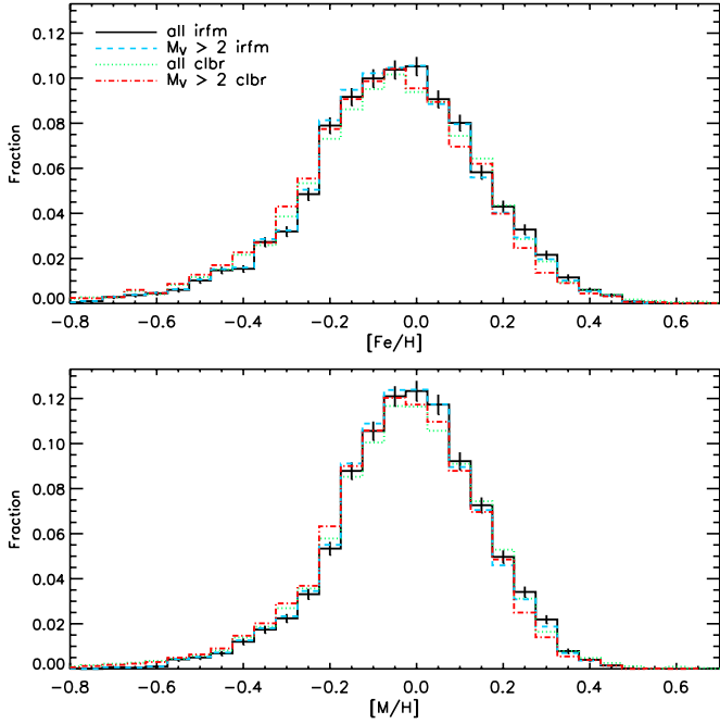
Fig. 15. MDF of the solar neighbourhood in terms of [\text{Fe}/\text{H}] ( upper panel ) and [\text{M}/\text{H}] ( lower panel ). Continuous line refers to stars belonging to the irfm sample (5976 stars within the colour ranges of the metallicity calibration), dashed line when considering only stars fainter than M_{V_T} = 2 , dotted line to all clbr stars (8470 within the colour ranges of the metallicity calibration) and dot-dashed when applying the same luminosity cut as above. Poisson error bars are shown for a representative case in both panels.
