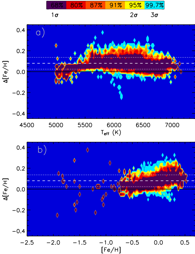
Fig. 6. \Delta[\text{Fe}/\text{H}] (in the sense ours minus GCSII) as function of T_{\text{eff}} (panel a ) and [\text{Fe}/\text{H}] (panel b ) for stars in the irfm sample satisfying the applicability range of our metallicity calibration. Notice the two breaks at 5500 K and 6500 K which correspond to the discontinuities introduced by the three calibrations used in GCSII for different (b - y) . Contour levels and lines as in Fig. 2.
