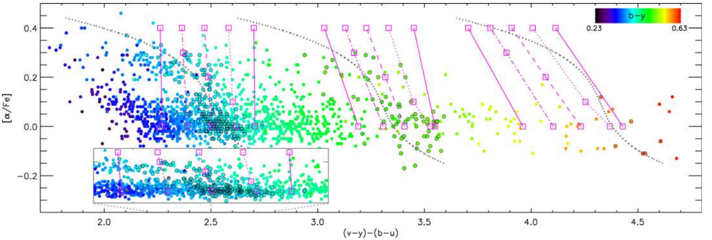
Fig. 9. [\alpha/Fe] versus (v-y)-(b-u) for our 1498 calibrating stars. Bluer (redder) colours indicate hotter (cooler) stars, according to their (b-y) , as shown in the top right box. Squares are synthetic colours computed from MARCS model fluxes at fixed [\alpha/Fe] (as available from MARCS library) for selected values of (b-y) = 0.4, 0.5, 0.6 (from left to right) and [Fe/H] = 0.00 dex with [\alpha/Fe] = 0 : 0.4 dex (continuous line) [Fe/H] = -0.25 dex with [\alpha/Fe] = 0:0.1:0.4 dex (dotted lines), [Fe/H] = -0.50 dex with [\alpha/Fe] = 0:0.2:0.4 dex (dashed lines), [Fe/H] = -0.75 dex with [\alpha/Fe] = 0:0.3:0.4 dex (dot-dashed lines), [Fe/H] = -1.00 dex with [\alpha/Fe] = 0:0.4 dex (triple-dot-dashed lines). Stars within 0.01 mag of the selected (b-y) interval are shown with open circles to highlight the trend. Grey dotted lines are fiducials built for those stars. Lower left panel is a zoom of the (b-y) = 0.4 data set for 2.2 \leq (v-y)-(b-u) \leq 2.8 .
