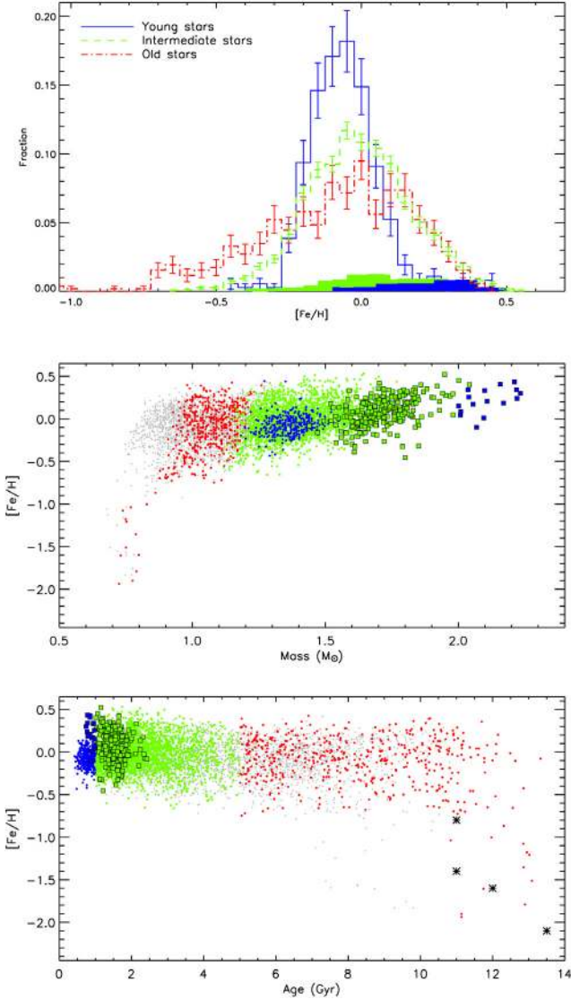
Fig. 16. Top panel: MDF for stars belonging to the irfm sample divided into different age intervals. Stars having age <1 Gyr are shown with a continuous line, 1 \leq \text{age} < 5 Gyr with a dashed line and age \geq 5 Gyr with a dot-dashed line. Shaded areas identify the subgroup of stars in the same age intervals as above, but with absolute magnitudes ( <2 ); no such bright stars are present in the old sample. Only stars with well determined ages (see Sect. 3) are used. Bars indicate Poisson errors. Middle panel: [\text{Fe}/\text{H}] versus stellar mass. Colours have the same meaning as in the top panel, with grey dots now referring to the remaining stars having more uncertain ages. Filled squares identify stars with bright absolute magnitudes ( <2 ). Lower panel: same symbols and colours as in the middle panel, but showing the age–metallicity relation. Shown for comparison (asterisks) are the ages and metallicities of the halo Globular Clusters studied in VandenBerg et al. (2010) (in the latter case, a different zeropoint on the age scale is possible, also depending on the input physics adopted in the stellar models employed).
