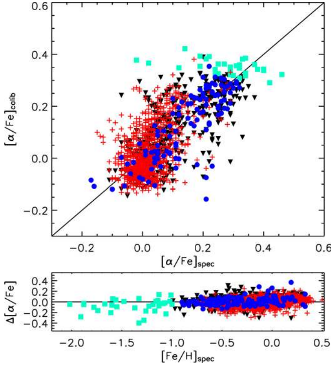
Fig. 10. Upper panel: spectroscopic versus Strömgen [\alpha/\text{Fe}] estimates for our 1498 calibrating stars. Crosses (circles) are stars having probability >90 percent of being thin (thick) disc based on their kinematic (using U, V, W velocities from the GCS). Downward triangles are stars with lower probability or for which kinematic information was not available. Filled squares are stars having [\text{Fe}/\text{H}] \leq -1 (independently of their kinematic thin/thick membership, if available). Lower panel: same symbols as above, showing the difference spectroscopic minus ours.
