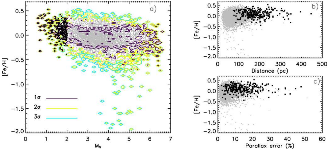
Fig. 8. Panel a) [Fe/H] distribution when slicing in absolute magnitude ( M_{V_T} ) 5976 stars (grey circles) that belong to the irfm sample and are within the metallicity calibration range. Contour levels are computed on abscissa intervals of 0.1 mag to equally represent regions with fewer stars. Panel b) and c) [Fe/H] distribution of the same stars, but plotted as a function of distance and parallax error. In all panels, stars with M_{V_T} < 2 are overlaid as black squares (271 in total).
