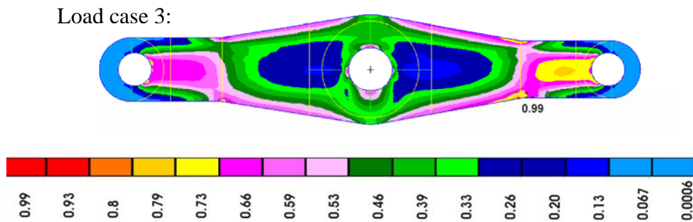
Figure 1.9: Distribution of the material efforts (load case 3)
