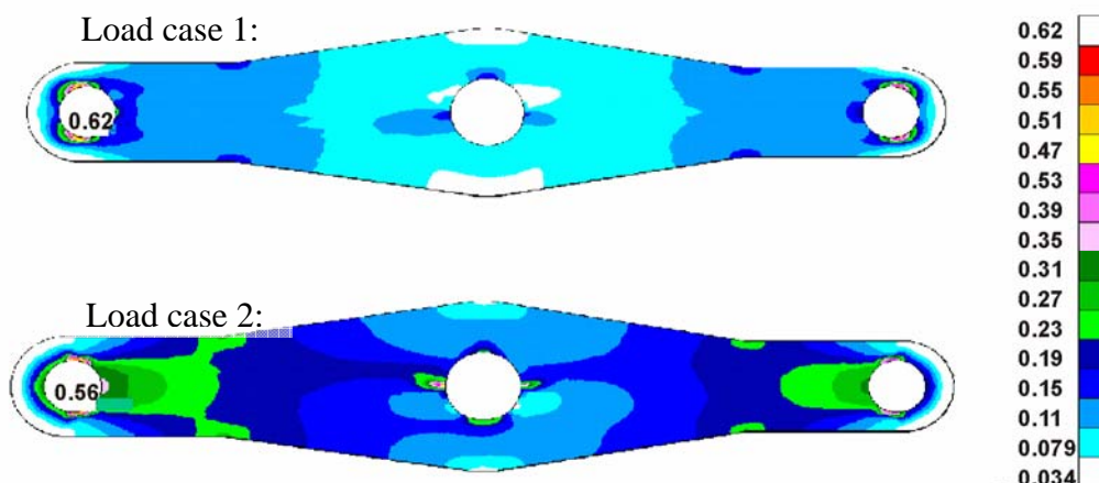
Figure 1.8: Distribution of the material efforts for load cases 1 and 2
