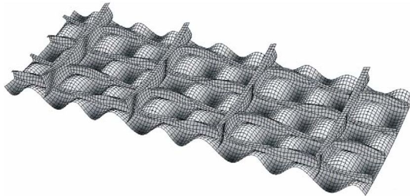
Figure 2.7: Deformed shape for Panel 2.
