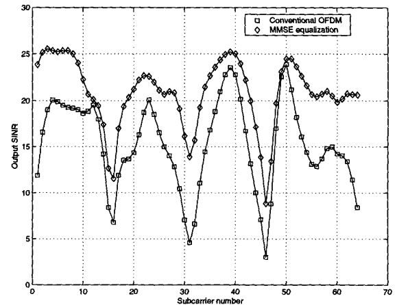
Figures 3: ( \square ) Signal-to-ICI-plus-noise ratio in conventional system, ( \diamond ) SNIR in new system as a function of subcarrier number for the channel in Figure 2.
