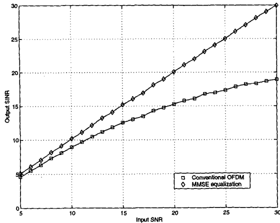
Figure 4: SINR before the slicer, versus input SINR for conventional OFDM receiver and our newly proposed system.
