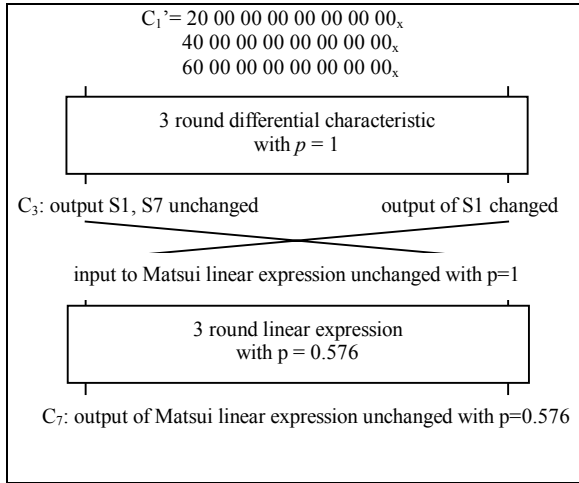
Figure 1. Differential-linear attack on DES reduced to 8 rounds
