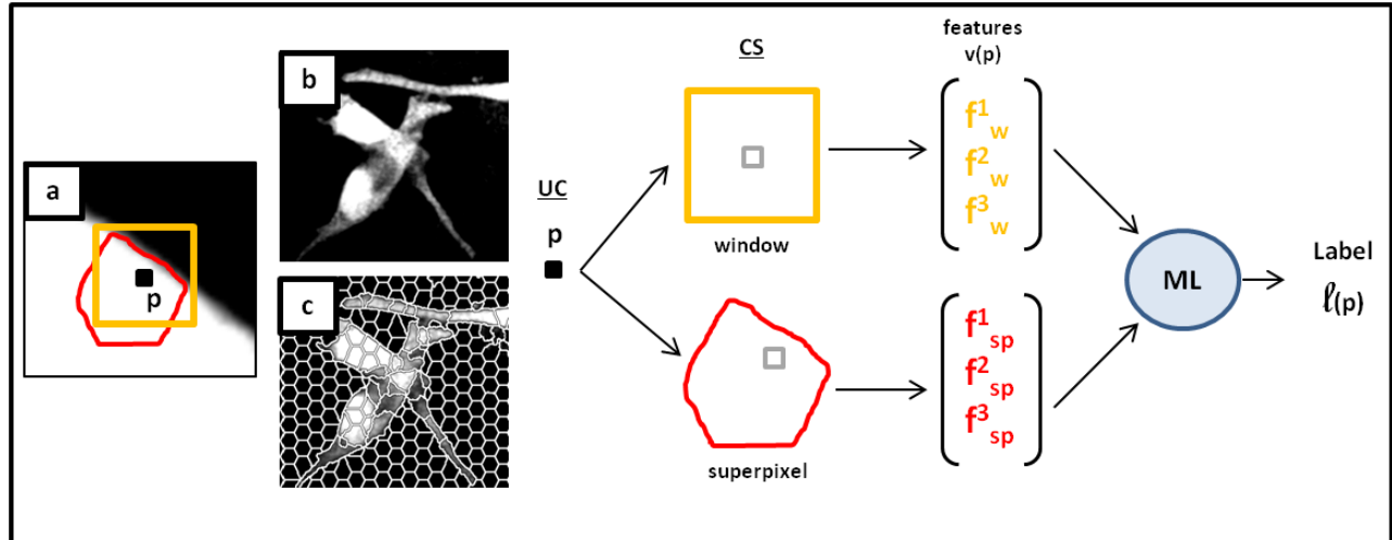
Fig. 1. Illustration of the proposed method : (a) regions for feature calculation (orange : sliding window, red : superpixel); (b) example image from the L'Oréal database (this image has been simplified for illustration purposes, see Fig.2 for a real case); (c) waterpixels (superpixels) computed on simplified image (b); computation of features on different computational supports, i.e. sliding window and superpixel, and their integration in the pixel's vector of features. "ML" : Machine Learning method .
