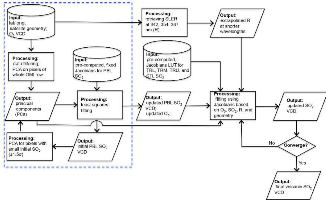
Figure 1. A flow chart of the new OMI volcanic \text{SO}_2 PCA retrieval algorithm (OMSO2VOLCANO). The first part of the algorithm, enclosed in the dashed blue box, is essentially identical to the operational OMI planetary boundary layer (PBL) \text{SO}_2 algorithm (Li et al., 2013) and provides input to the second part of algorithm that performs iterative spectral fitting to retrieve volcanic \text{SO}_2 VCD.
