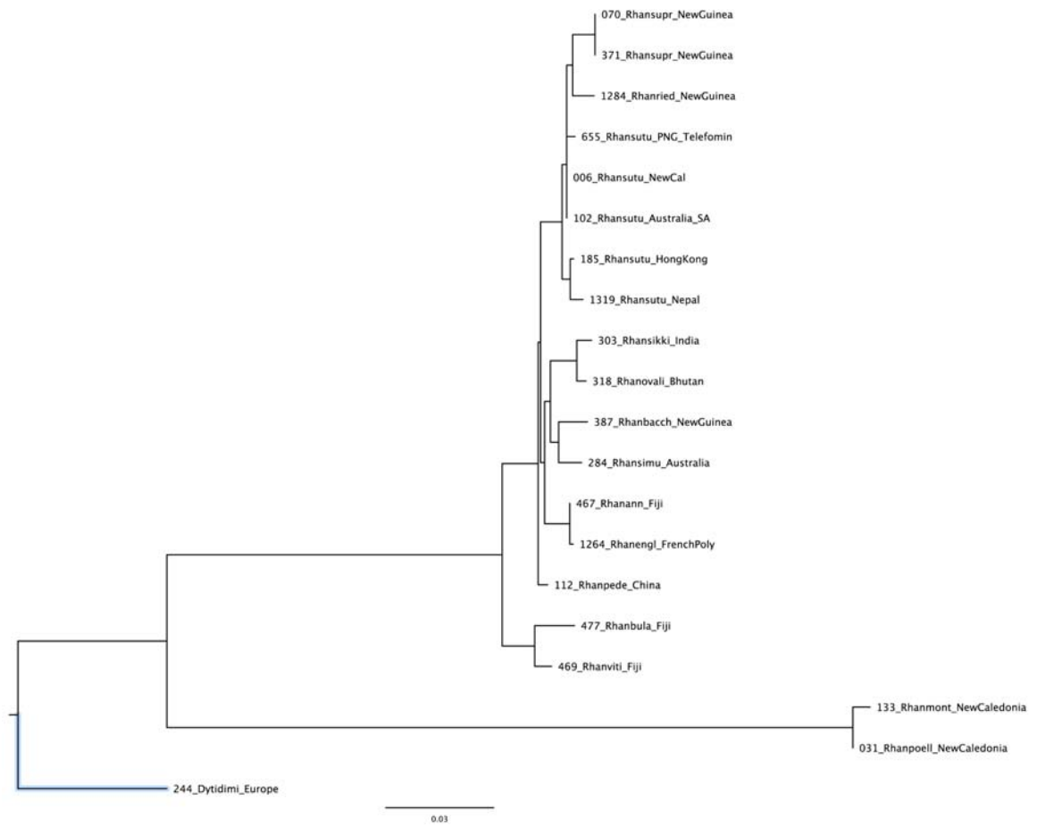
ESM Fig. S2 C. Maximum likelihood analysis using Garli, of EF1 \alpha exons only.
