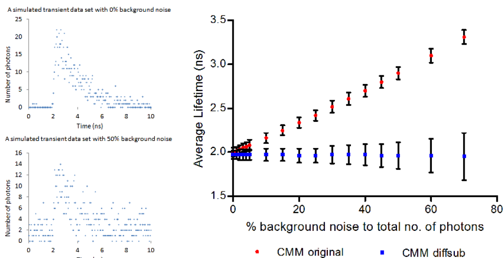
Fig. 7. Analysis of simulated transient data sets showing how increasing the percentage contribution background noise to total number of photons affected the average lifetime value of 4096 transients determined using CMM original and CMM diffsub . For each individual transient, the total number of photons remains constant at 1000 counts.
