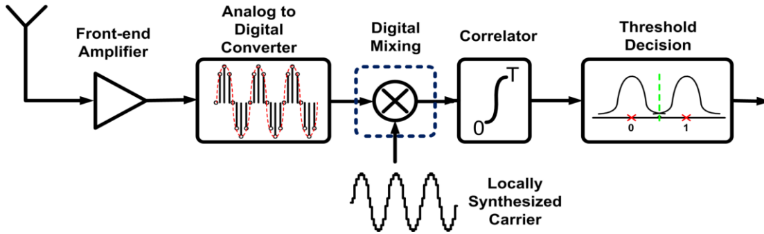
Figure 11. A digital receiver architecture for BPSK.
