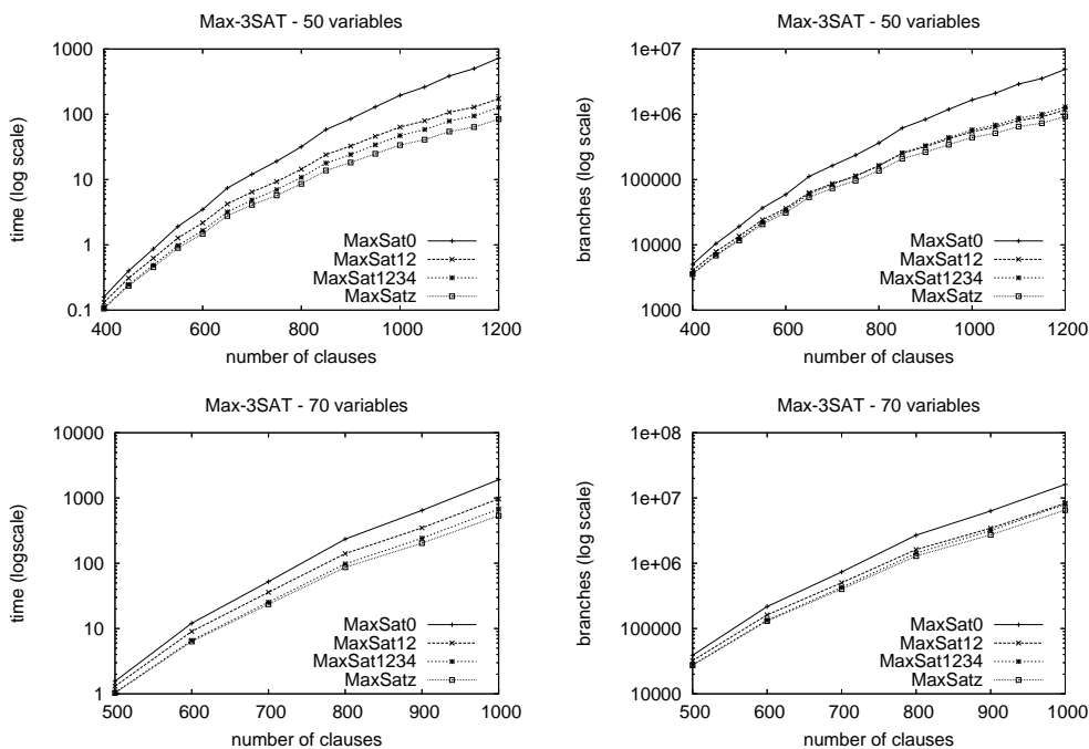
Figure 8: Comparison among MaxSat12, MaxSat1234 and MaxSatz on random Max-3SAT instances.
