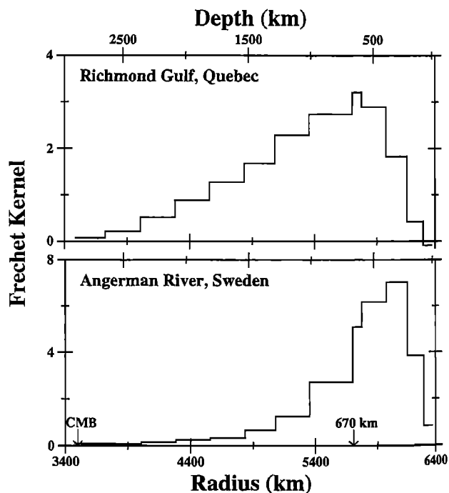
Fig. 2. Frechet kernels for the numerical prediction of the decay time associated with post-glacial RSL variations at Richmond Gulf and Angerman River. The calculations adopt the ‘TP’ viscosity profile given in Fig. 3a (dashed line).
