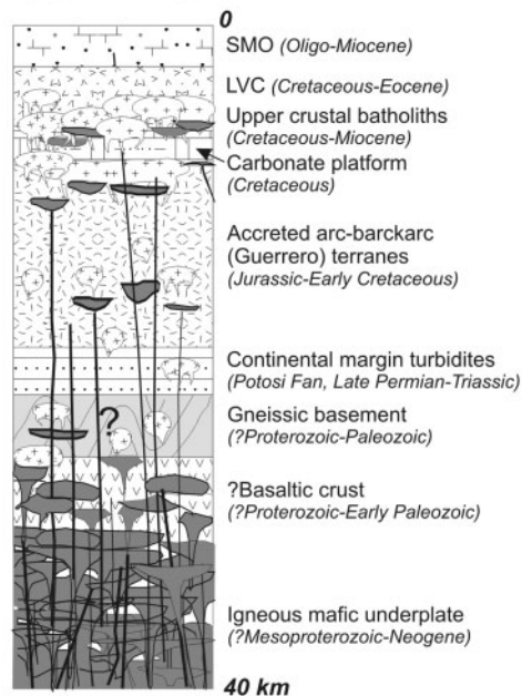
Fig. 2. Schematic crustal sections showing the inferred architecture, age and composition of the crust beneath the northern, central and southern SMO (see inset), based on Centeno-García et al. (2007), Ferrari et al. (2007) and Housh & McDowell (2007), and references therein. The thickness of each crustal section is based on Bonner & Herrin (1999) for the northern SMO, and Couch et al. (1991) for the central and southern SMO. The thicknesses of the component crustal units are not to scale. States mentioned in text are shown in the inset map. LVC, Lower Volcanic Complex; Zac, Zacatecas; Gua, Guanajuato; SLP, San Luis Potosi.
