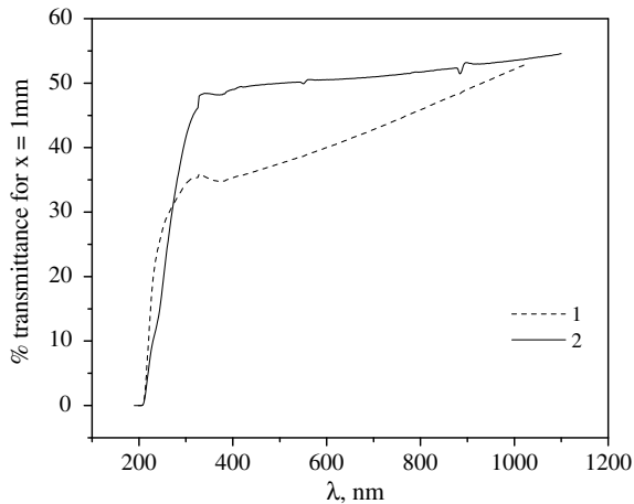
Fig. 14. Transmission spectra of partly crystallized glass of composition TGC-2 containing about 42% crystal phase by single (2) and double (1) heat treatments, having crystal number densities about 1.2 \cdot 10^4 and 2 \cdot 10^6 \text{ mm}^{-3} and crystal diameters of 47 and 7.5 \mu\text{m} , respectively.
