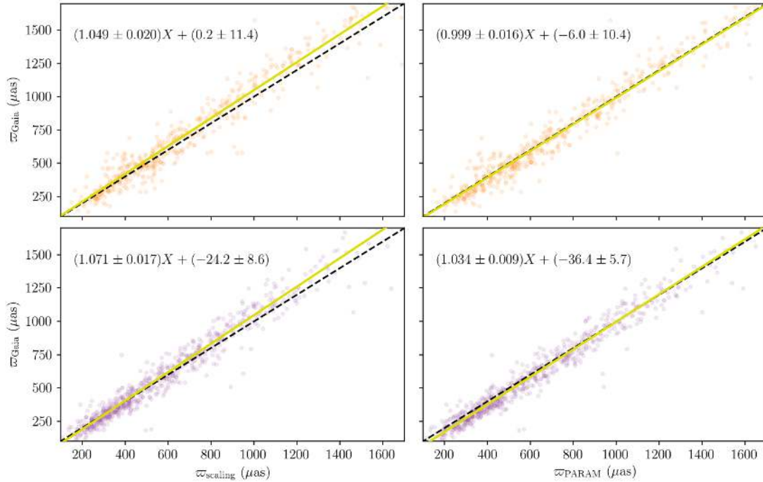
Fig. 11. \sigma_{Gaia} as a function of \sigma_{scaling} (left) and \sigma_{PARAM} (right) for red giants in the K2 Campaign fields C3 (top) and C6 (bottom). The yellow line displays the linear fit, averaged over N realisations, for which the relation is given at the top of each subplot. The black dashed line indicates the 1:1 relation. The summary statistics are: (\overline{\Delta\sigma})_m = 28.9 \pm 5.2 \mu\text{as} , (\overline{\Delta\sigma})_w = 24.6 \pm 4.0 \mu\text{as} , and z = 1.16 for C3 (scaling); (\overline{\Delta\sigma})_m = 11.9 \pm 3.6 \mu\text{as} , (\overline{\Delta\sigma})_w = 9.5 \pm 2.6 \mu\text{as} , and z = 1.01 for C6 (scaling); (\overline{\Delta\sigma})_m = -8.1 \pm 4.4 \mu\text{as} , (\overline{\Delta\sigma})_w = -6.4 \pm 3.8 \mu\text{as} , and z = 1.30 for C3 (PARAM); (\overline{\Delta\sigma})_m = -18.6 \pm 3.3 \mu\text{as} , (\overline{\Delta\sigma})_w = -16.9 \pm 2.4 \mu\text{as} , and z = 1.11 for C6 (PARAM).
