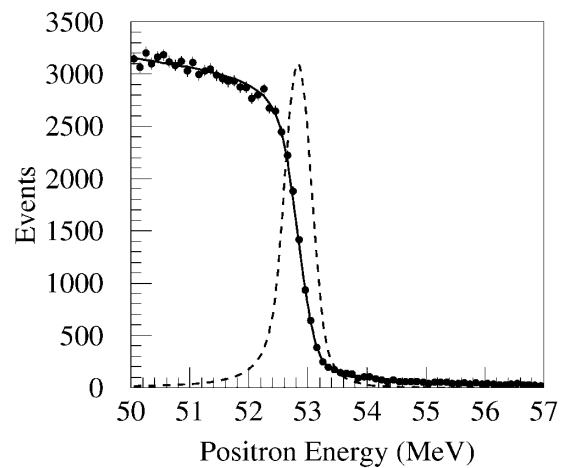
FIG. 3. The E_e spectrum from \mu^+ \rightarrow e^+ \nu \bar{\nu} extracted from full rate data for the middle topology group. The solid curve is the fit used to extract the line shape (dashed curve).
