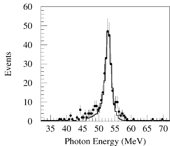
FIG. 1. The E_\gamma spectrum from photons converting in the outer layer of lead. The data points are produced by stopping pions in \text{CH}_2 via the reaction \pi^- p \rightarrow \pi^0 n \rightarrow \gamma\gamma n , scaled from 54.9 to 52.8 MeV. The curve is the response function generated from the MC and used in the analysis of the \mu^+ \rightarrow e^+\gamma data.
