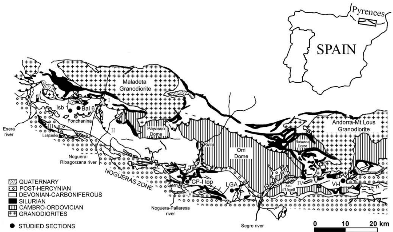
Fig. 1.- Geological scheme of the study area in the Central Spanish Pyrenees, indicating the four Subfacies areas contained in the Palaeozoic outcrops in the Southern Facies-area of Mey (1967): I) Sierra Negra Subfacies, II) Baliera Subfacies, III) Renanué Subfacies and IV) Compte Subfacies; together with the location of the seven sections studied: Isábena I section (Isb 1), Baliera 6 section (Bal), the LGA X and LGA XI sections (LGA), Compte-I top section. (CP-I top) and Villech IA section (Vi-I) (Based on Valenzuela-Ríos, 1994).
