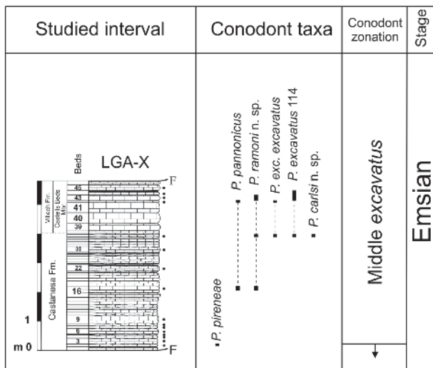
Fig. 4-. Stratigraphic column of the LGA X section showing the location of the levels sampled for conodonts (black dots) and ranges of selected conodont taxa. The age of the bottom of the section is given by unpublished data from the genus Icriodus .
