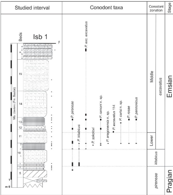
Fig. 3-. Stratigraphic column of the Isábena 1 section showing the location of the levels sampled for conodonts (black dots) and ranges of selected conodont taxa.
