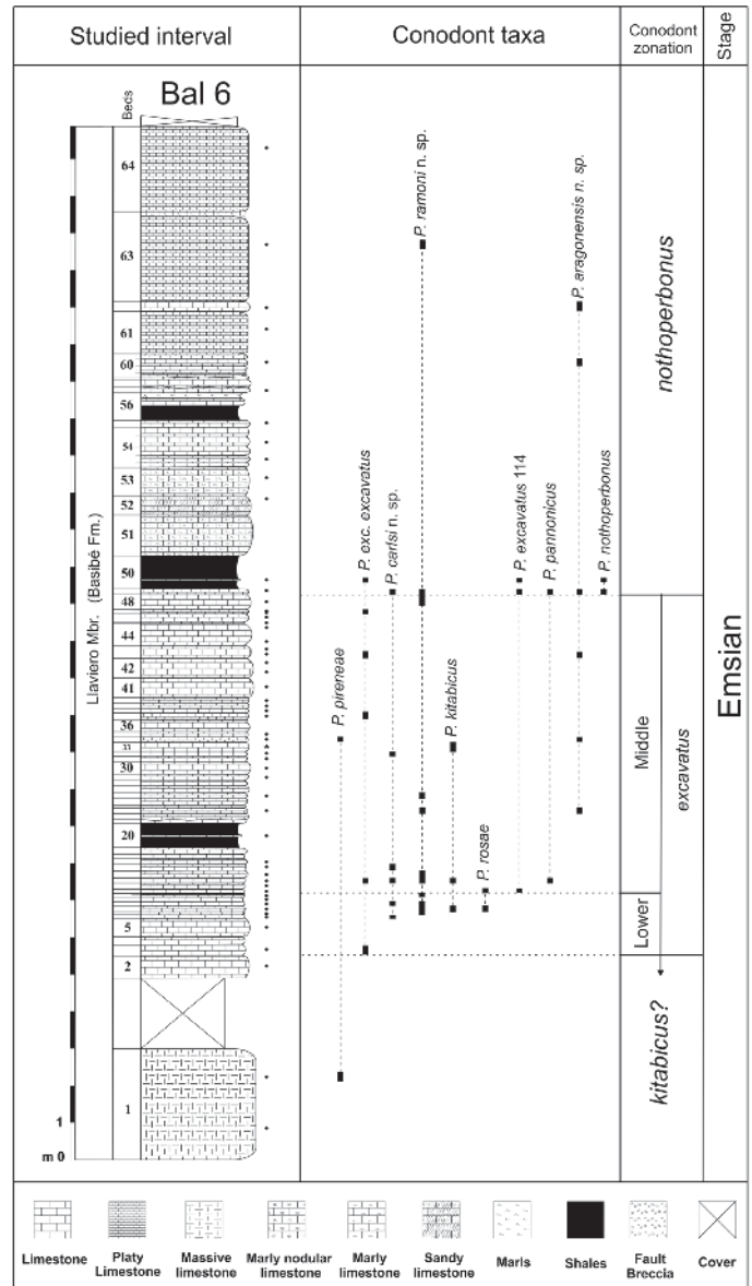
Fig. 2-. Stratigraphic column of the Baliera 6 section showing the location of the levels sampled for conodonts (black dots) and ranges of selected conodont taxa of biostratigraphic relevance. Polygnathus notoperbonus is just figured to show the upper boundary of the Middle excavatus Zone.
