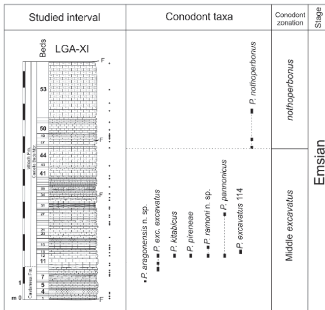
Fig. 5-. Stratigraphic column of the LGA-XI section showing the location of the levels sampled for conodonts (black dots) and ranges of selected conodont taxa. Polygnathus nothoperbonus is just figured to show the upper boundary of the Middle excavatus Zone. The age of the bottom of the section is given by lithological correlation with the top of the LGA-X section.
