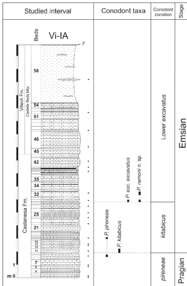
Fig. 7-. Stratigraphic column of the Vi-IA section showing the location of the levels sampled for conodonts (black dots) and ranges of selected conodont taxa.
