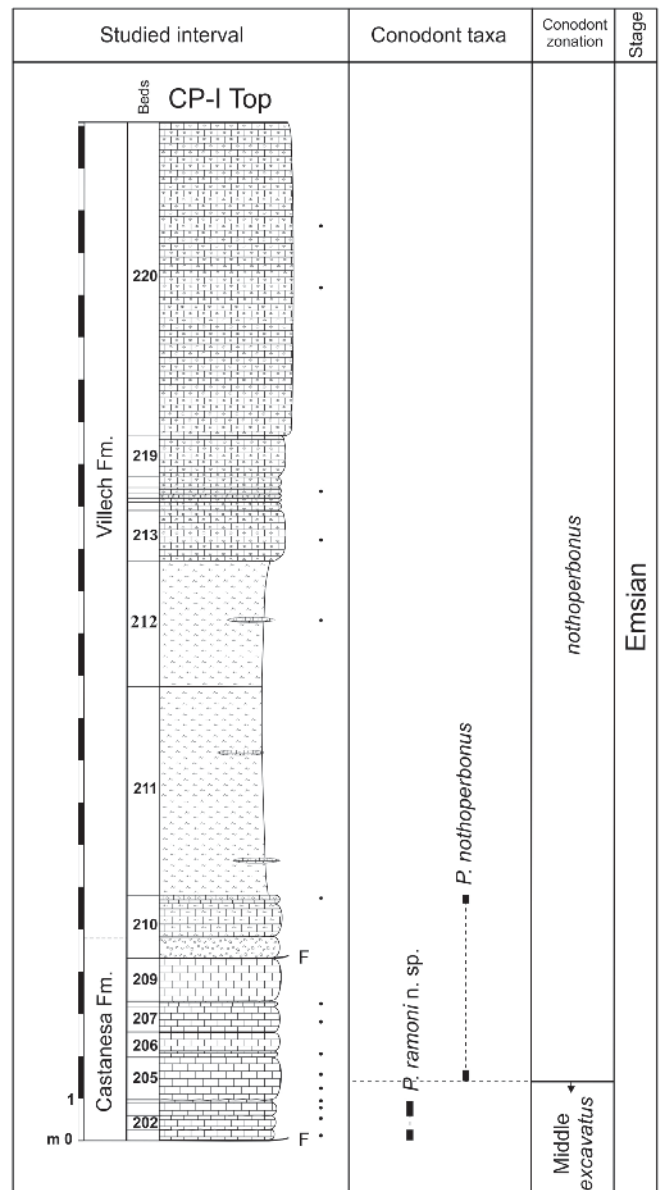
Fig. 6-. Stratigraphic column of the CP-I top section showing the location of the levels sampled for conodonts (black dots) and ranges of selected conodont taxa. Polygnathus nothoperbonus is just figured to show the upper boundary of the Middle excavatus Zone.
