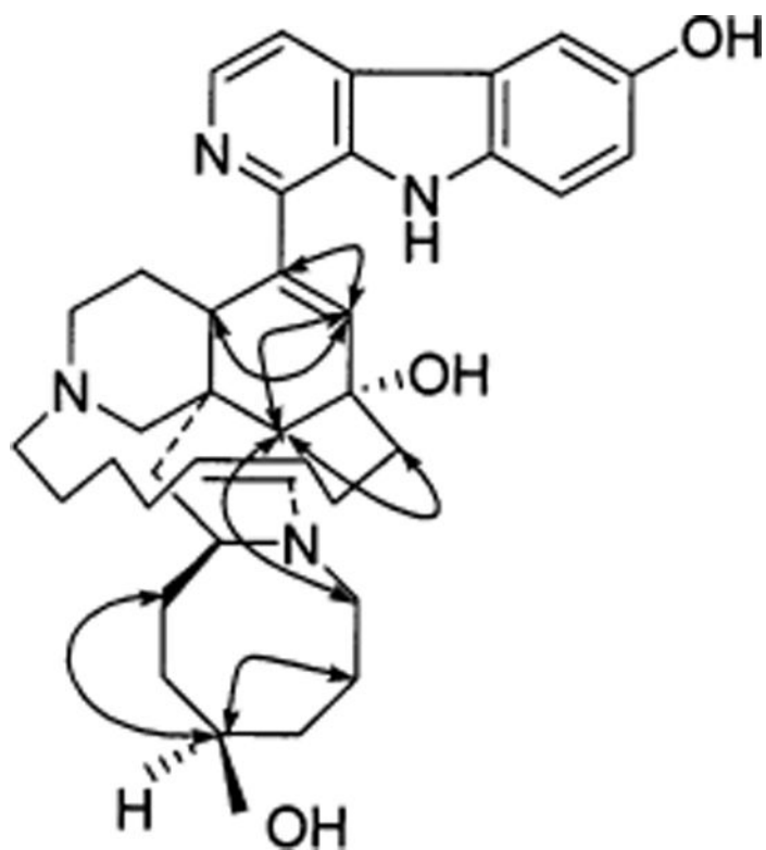
Figure 3. Selected HMBC correlations of 7.
