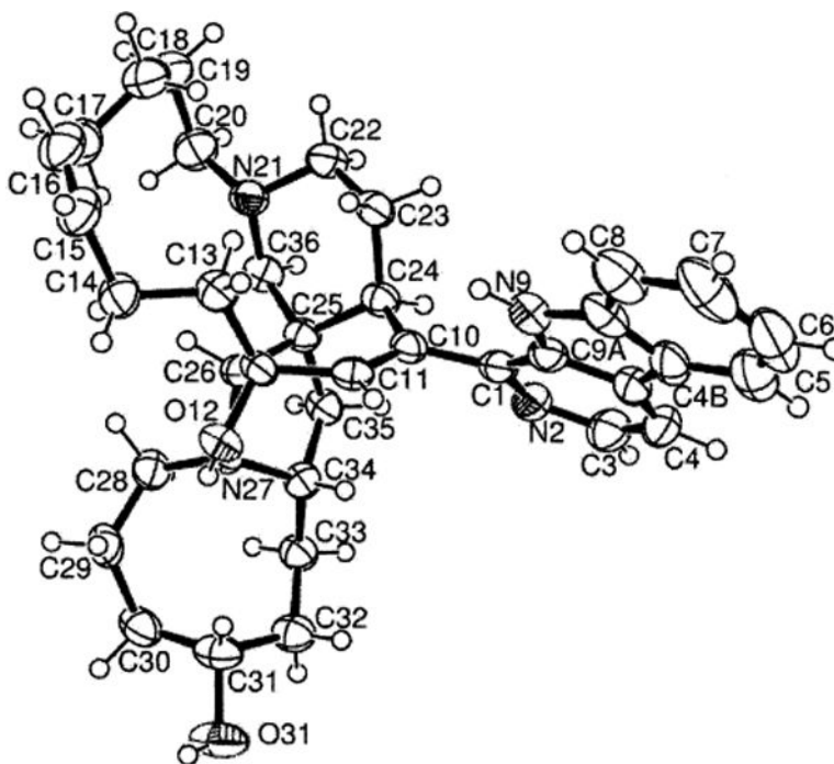
Figure 4. ORTEP24 drawing of one independent molecule in compound 3 . For simplicity, the numbering scheme used for the X-ray structure depicts connectivity and does not follow the standard IUPAC convention.
