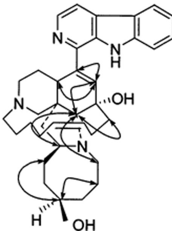
Figure 1. Selected HMBC correlations of 3.
