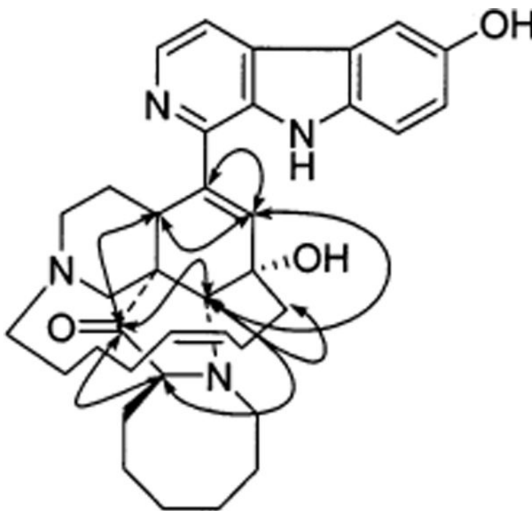
Figure 2. Selected HMBC correlations of 5.
