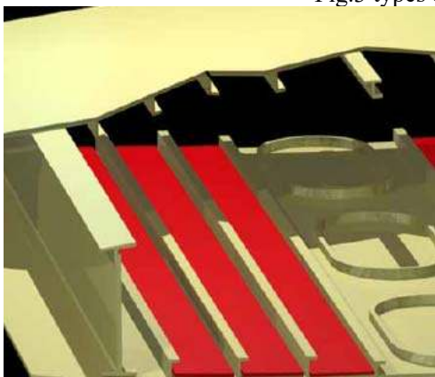
Fig. 4 Integral stiffened panels
