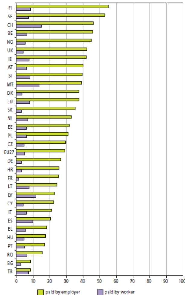
Figure 5: Employee training (2005-2006):
