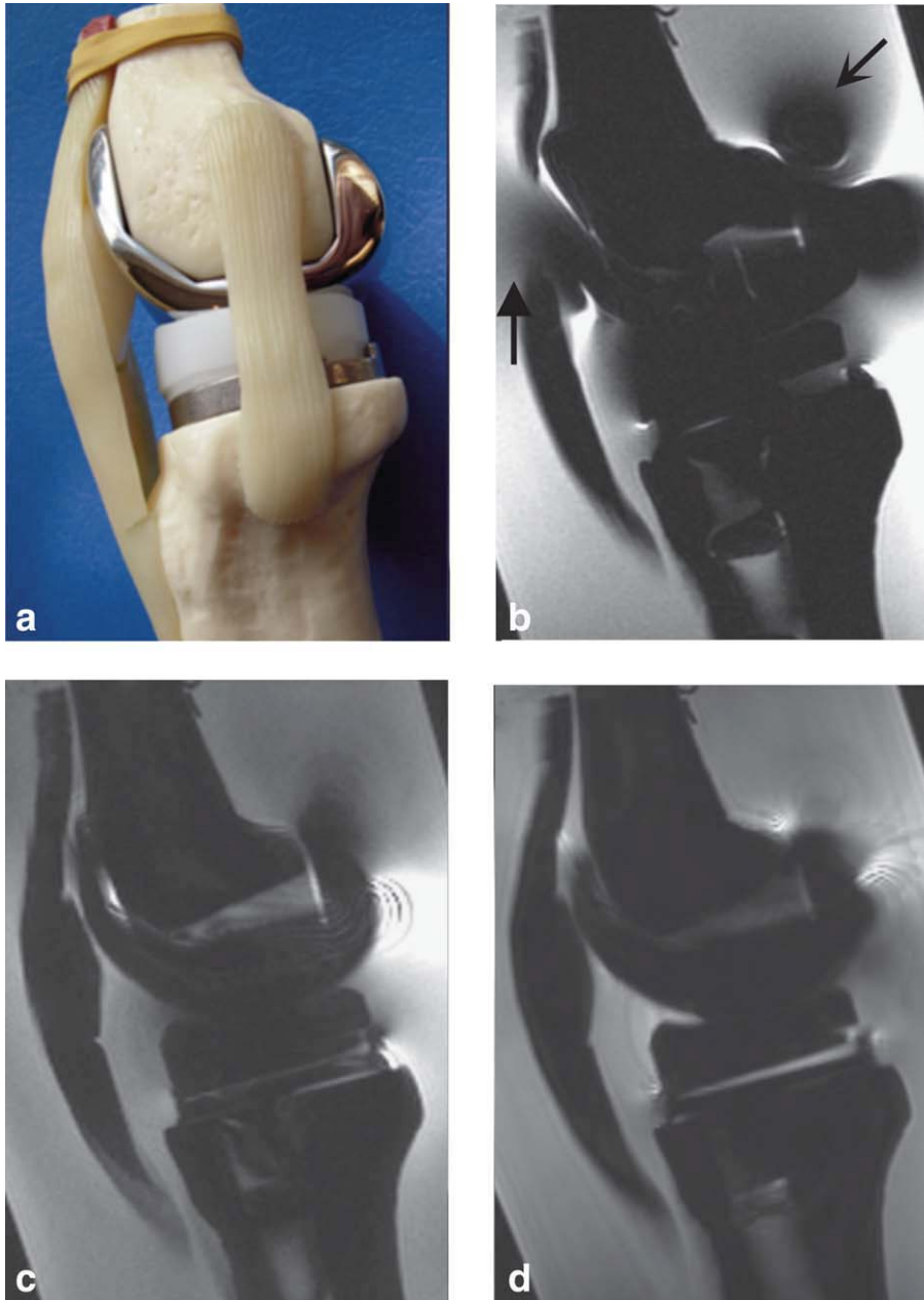
Figure 3. Sagittal view (a) of the custom-made model of the postoperative knee, consisting of plastic femoral and tibial bones (Zimmer, Warsaw, IN) filled with oil to simulate subchondral fat, and fitted to standard TKR components (Zimmer NexGen LPS-Flex cobalt-chrome femoral component, polyethylene spacer, and Zimmer NexGen MIS Mini-Keel titanium tibial component). Water doped with copper sulfate surrounding the knee model simulates the MR relaxation properties of adjacent tissue in the knee. Sagittal MR imaging of the TKR knee model shows that FSE (b) had severe metal-induced distortion (wedge-shaped arrow) and signal loss (curved arrow) in comparison to SEMAC (c) and MAVRIC (d) images. [Color figure can be viewed in the online issue, which is available at wileyonlinelibrary.com .]
