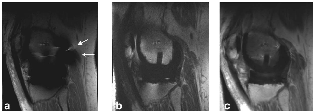
Figure 1. Sagittal MR images of a TKR in a healthy volunteer. Metal-induced artifact including distortion (wedge-shaped arrow) and signal loss (curved arrow) severely limit the diagnostic value of FSE (a) images. SEMAC (b) and MAVRIC (c) correct for the artifact, allowing easier visualization of adjacent bone and soft tissue structures.
