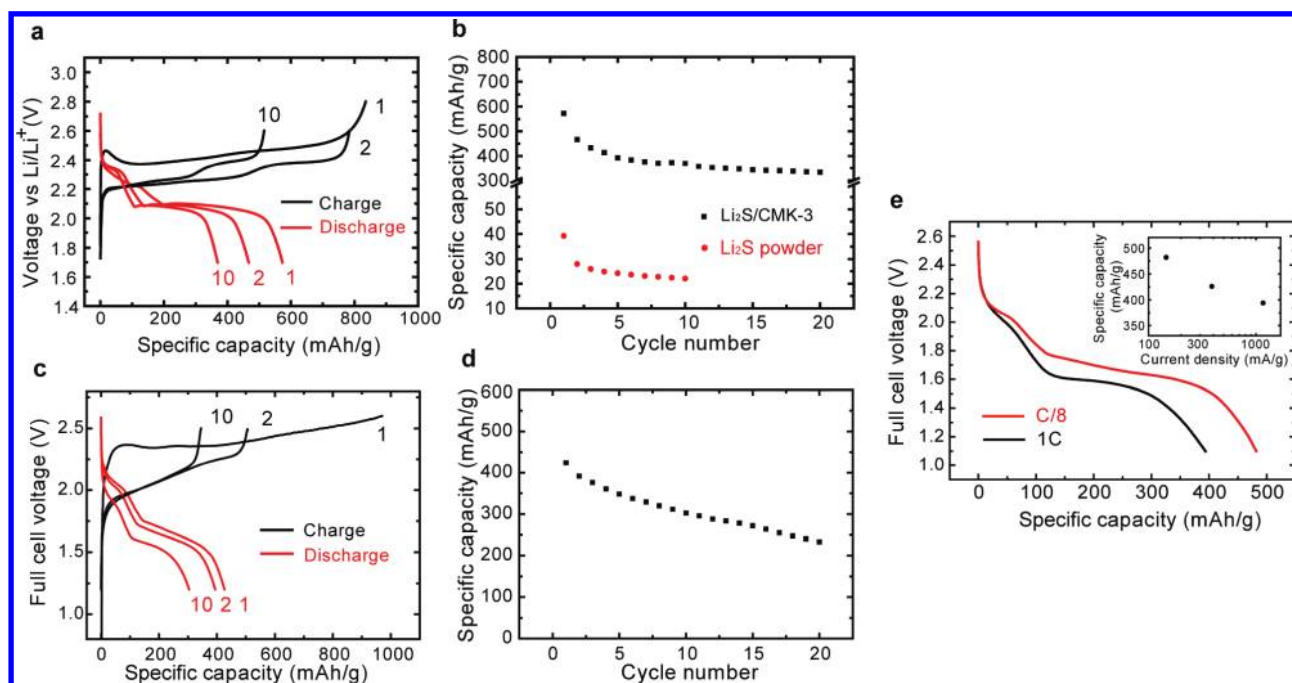
FIGURE 4. Electrochemical tests of Li 2 S/Li half-cells and Li 2 S/Si full cells. All specific capacity values are given with respect to the mass of Li 2 S. (a,b) Voltage profile (a) and specific discharge capacity with cycling (b) of a Li 2 S/CMK-3 mesoporous carbon nanocomposite half-cell containing a lithium counter electrode. The current rate is C/8 (146 mA g -1 ) and the voltage range is 1.7–2.8 V for the first cycle and 1.7–2.6 V for following cycles. The specific discharge capacity with cycling of a Li 2 S commercial powder half-cell is also shown for comparison in (b). (c,d) Voltage profile (c) and specific discharge capacity with cycling (d) of a full battery cell with a Li 2 S/CMK-3 mesoporous carbon nanocomposite cathode and a silicon nanowire anode. The current rate is C/3 (389 mA g -1 ) and the voltage range for the full cell is 1.2–2.6 V for the first cycle and 1.2–2.5 V for following cycles. (e) First discharge voltage profiles of full battery cells with Li 2 S/CMK-3 mesoporous carbon nanocomposite cathodes and silicon nanowire anodes at rates of 1C (1166 mA g -1 ) and C/8 (146 mA g -1 ). The inset in (e) is a plot of the first discharge specific capacity of full cells operating at various current rates.
