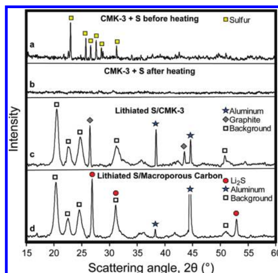
FIGURE 3. X-ray diffraction characterization of \text{Li}_2\text{S}/\text{mesoporous carbon nanocomposite particles} . (a,b) Scan of a mixture of sulfur and CMK-3 mesoporous carbon powder before heating (a) and after heating at 155\text{ }^\circ\text{C} (b). (c) Scan of sulfur/CMK-3 mesoporous carbon nanocomposite lithiated by reaction with n -butyllithium and heated at 105\text{ }^\circ\text{C} . The aluminum and graphite peaks are due to the carbon-coated aluminum foil substrate. (d) Scan of a sulfur/macroporous carbon nanocomposite lithiated by reaction with n -butyllithium and heated at 105\text{ }^\circ\text{C} . The aluminum peaks are due to the aluminum foil substrate. The peaks labeled “Background” in c and d result from a protective cover used to prevent oxidation. Peaks are identified with the following symbols: yellow square, sulfur; blue star, aluminum; gray diamond, graphite; open square, background; red circle, \text{Li}_2\text{S} .
