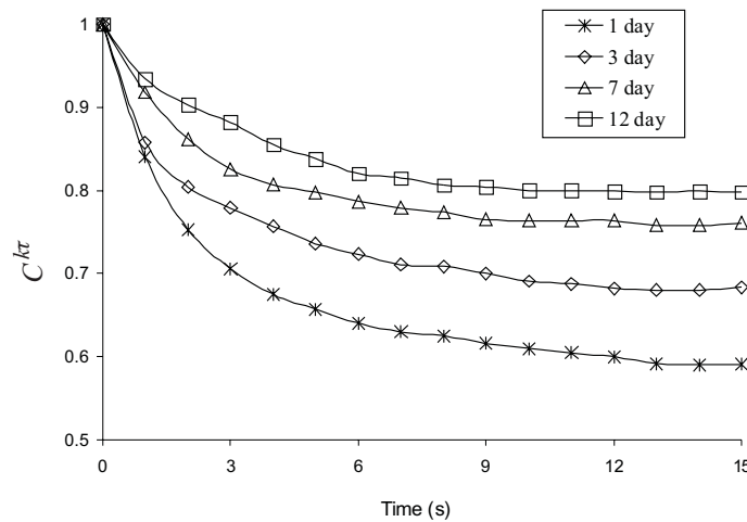
Fig. 4. Temporal changes of cross-correlation coefficients for apple surface during shelf-life storage (12 days).
