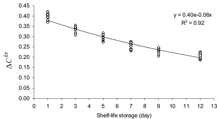
Fig. 5. The cross-correlation coefficient value difference \Delta C^{kr} in a function of storage day (shelf-life).
