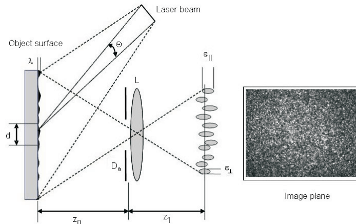
Fig. 1. Creation of the subjective speckle pattern.
