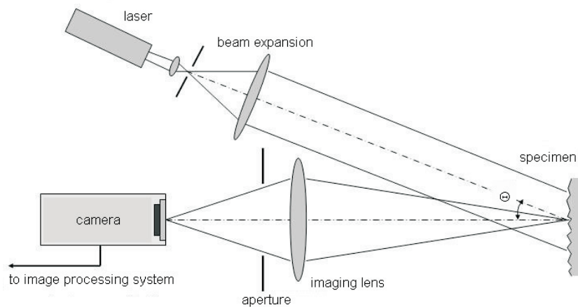
Fig. 2. Experimental setup for Digital Speckle Correlation system.
