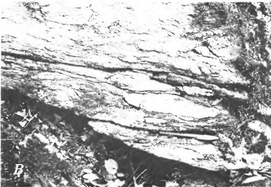
Figure 9. Quartzite boulders in deformed conglomerate along Hamann Creek. A , Relatively undeformed conglomerate with abundant volcanic clasts in the matrix. B , Flattened quartzite boulders in conglomerate about 30 m from locality of A .
