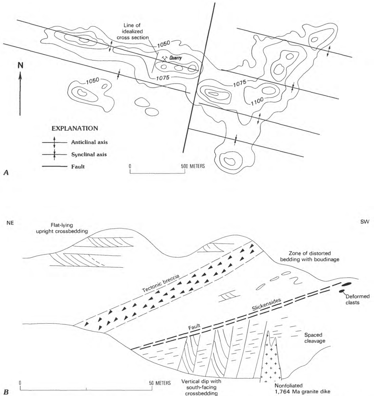
Figure 2. Map and cross section of Hamilton Mounds area. A, Topographic hills (contoured in feet) and N. 75° W.-trending anticline and syncline axes (modified from Ostrander, 1931). B, Diagrammatic cross section showing major lithologic and structural features at the main quarry in the Hamilton Mounds area. Location of cross section is shown in A. Vertical scale exaggerated.
