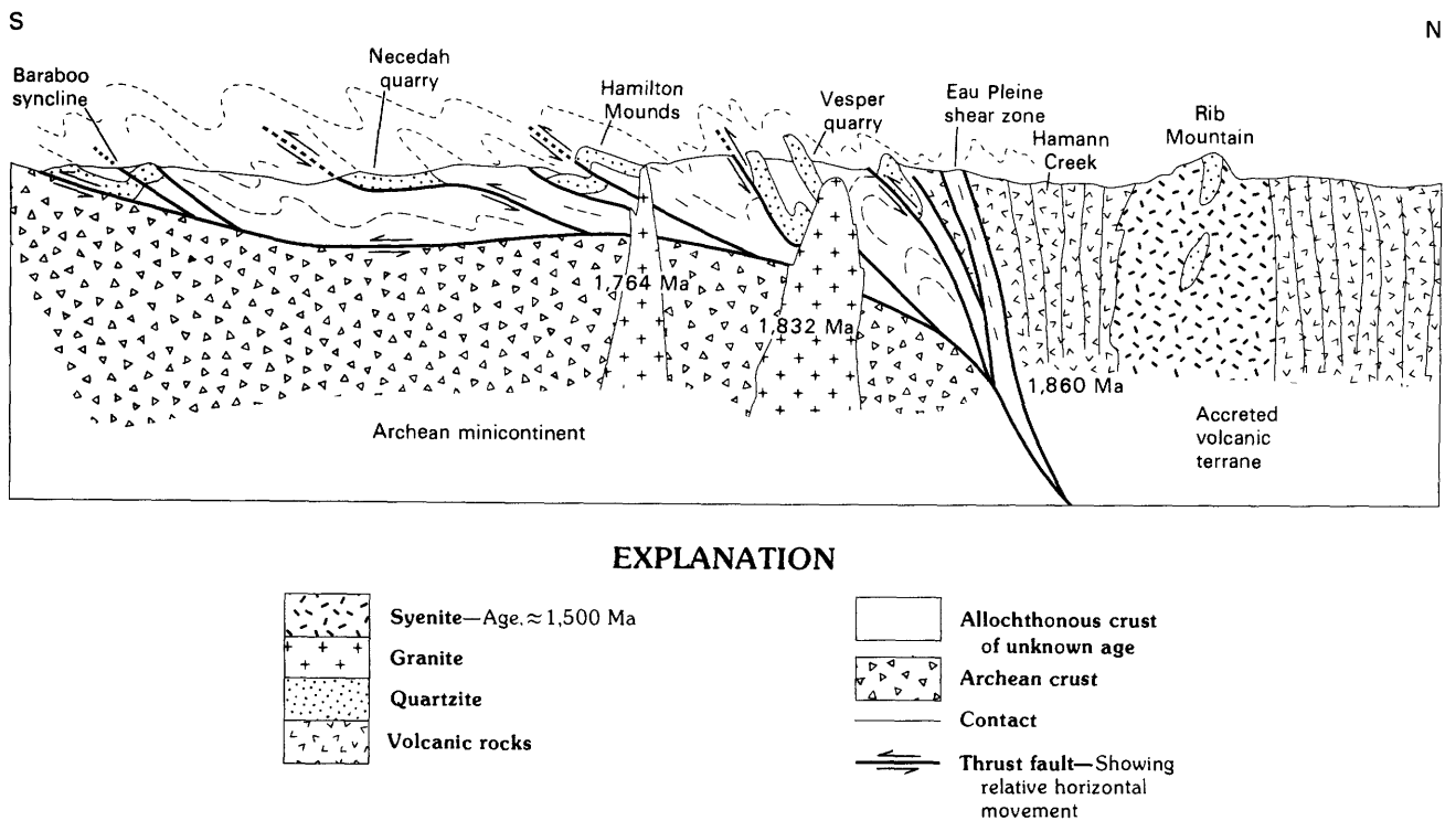
Figure 12. Interpretive sketch of tectonic relationships of the quartzites in central and southern Wisconsin, illustrating nature of proposed south-verging deformation. Length of section \approx 175 km. Vertical, not to scale.
