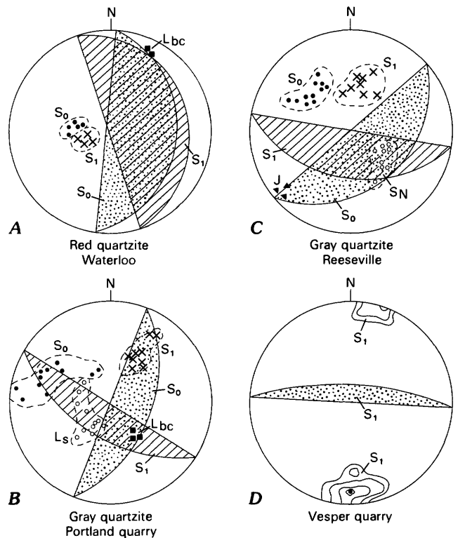
Figure 7. Lower hemisphere plots of structural data from Waterloo and Vesper areas. A , Red quartzite at Waterloo. Solid dots and stippled plane indicate orientation of bedding ( S_0 ); x and lined plane indicate orientation of cleavage ( S_1 ) in thin pelitic layers. Solid squares are measured lineations formed by intersection of cleavage and bedding ( L_{bc} ). B , Gray quartzite at Portland quarry. Solid dot, pole to bedding ( S_0 ); stippled plane, approximate orientation of bedding; x, pole to spaced cleavage ( S_1 ); lined plane, approximate orientation of spaced cleavage ( S_1 ) in quartzite. Solid square, orientation of lineation (intersection of bedding and cleavage, L_{bc} ). Open circle, orientation of long axis of stretched clast ( L_c ). C , Gray quartzite near Reeseville. Solid dot, pole to bedding; stippled plane, approximate orientation of bedding ( S_0 ); x, pole to S_1 foliation; lined plane, approximate orientation of joints (J); solid triangle, pole showing orientation of joints (J); open circle, pole to a spaced cleavage/joint system ( S_N ). D , Stereoplot of spaced cleavage in quartzite at Vesper quarry. Contours 5, 10, 20 percent are on 21 poles to cleavage ( S_1 ). Solid dot, area of highest concentration. Stippled plane, orientation of S_1 cleavage.
