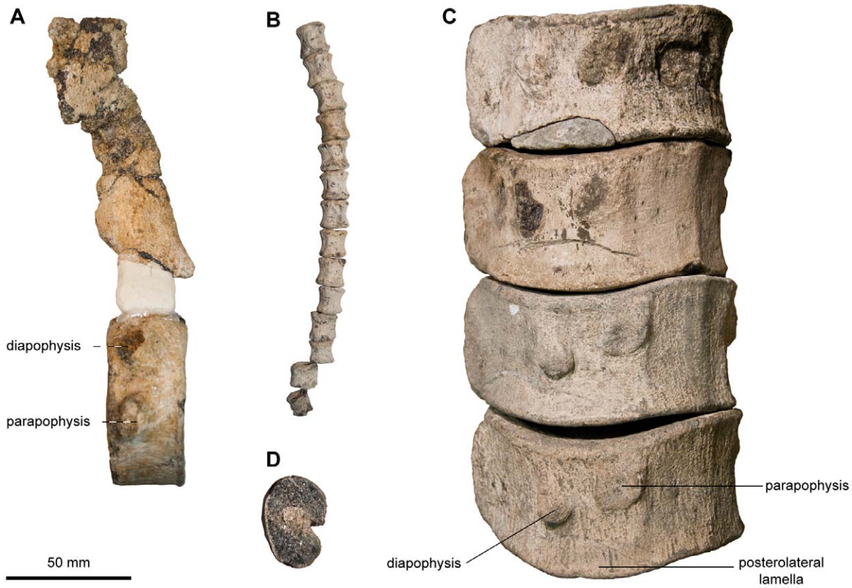
Figure 7. Diagnostic features of the axial skeleton of Acamptonectes densus . A: anterior dorsal centrum and associated neural spine of SNHM1284-R, showing the large size of the neural spine with respect to the centrum height. B: series of posterior postflexural centra of SNHM1284-R showing their square shape ( H/L \approx 1 ). C: series of posterior dorsal centra of GLAHM 132588 (holotype), showing the markedly curved profile of the posterolateral lamella. D: cross-section of a rib of NHMUK R11185 showing their robust morphology and the minute groove occurring on one side only. doi:10.1371/journal.pone.0029234.g007
