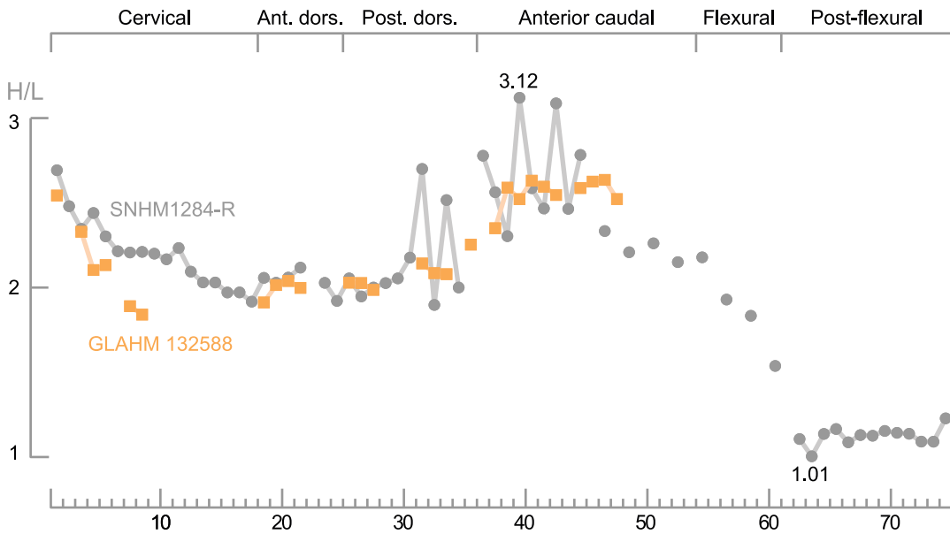
Figure 8. Regionalization of the vertebral column in Acamptonectes densus . Both specimens have incomplete vertebral series and the centra were therefore superposed manually in each region, using the centrum shape and relative position of the apophyses. Each obvious gap in the vertebral column is represented by a single void in the series of SNHM1284-R. The x-axis refers to the centrum count, not its actual position within the vertebral column. The regionalization of the vertebral column is quite weak, in between that of Sveltonectes insolitus [34] and Ophthalmosaurus icenicus [69]. doi:10.1371/journal.pone.0029234.g008
