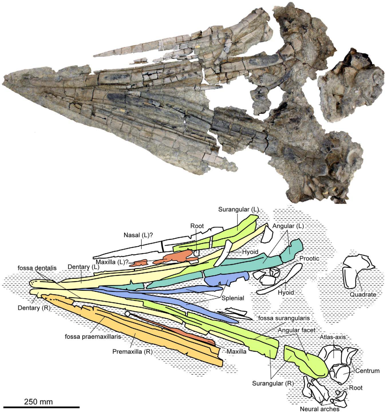
Figure 1. Skull and partial cervical region of Acamptoneustes densus (SNHM1284-R). doi:10.1371/journal.pone.0029234.g001
