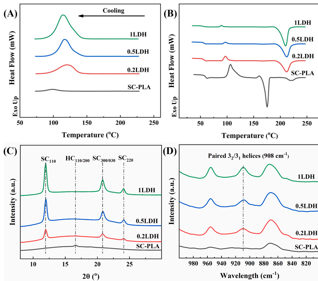
Fig. 1. Heat flow of SC-PLA nanocomposite films with various LDH content measured during (A) cooling from 250 \text{ }^\circ\text{C} to 30 \text{ }^\circ\text{C} at 10 \text{ }^\circ\text{C}/\text{min} and (B) subsequent heating to 250 \text{ }^\circ\text{C} at 10 \text{ }^\circ\text{C}/\text{min} , and corresponding X-ray diffraction (C) and FTIR spectra (D) of the nanocomposite after the nonisothermal crystallization cooling from 250 \text{ }^\circ\text{C} to 30 \text{ }^\circ\text{C} .
