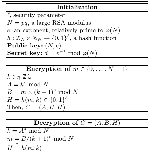
Fig. 2. First Variant: The DRSA-1 Encryption Scheme
