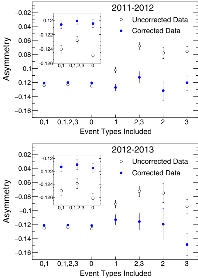
FIG. 5. Corrected and uncorrected asymmetries for various combinations of event types. Only \Delta_{\text{backscattering}} and \Delta_{\text{cos}\theta} are applied and error bars are statistical only. The first three combinations include Type 0 events which are identified as having not backscattered and make up roughly 95% of the data. The remaining four asymmetries include only the various backscattering events. The inset shows a closer view of the first three points whose error bars are smaller than the markers in the larger plot. Top: 2011–2012. Bottom: 2012–2013.
