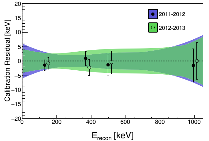
FIG. 3. Plot of energy uncertainty vs. reconstructed energy. The points plotted are the mean and \sigma of the residual distributions from reconstructed calibration peaks of Ce, Sn, and the lower and upper Bi peaks in that order. The bands represent the energy uncertainty at any given electron energy for the two data sets.
