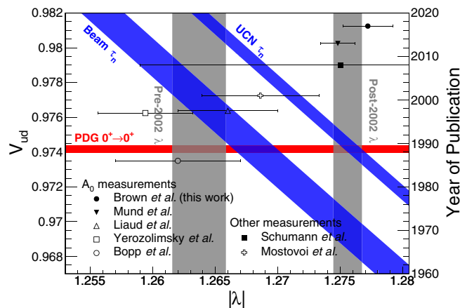
FIG. 6. Status of V_{ud} , the neutron lifetime, and \lambda measurements. The \lambda result bands (vertical) are divided into pre-2002 [40–42] and post-2002 [18,44–46] results, where the distinction is made using the date of the most recent result from each experiment. The right axis shows publication year for the individual lambda measurements included in the calculation of the \lambda bands (closed markers for post-2002, open markers for pre-2002). Note that the result of this work (Brown et al. ) is the combined UCNA result from [18] and the current analysis, and the Mund et al. result is the combined PERKEO II result from [43,44]. The diagonal bands are derived from neutron lifetime measurements and are separated into neutron beam [31,32] and UCN bottle experiments, which consist of material bottle storage [34–38] and magnetic bottle storage [33]. The V_{ud} band (horizontal) comes from superallowed 0^+ \rightarrow 0^+ nuclear \beta -decay measurements [39]. The error bands include scale factors as prescribed by the Particle Data Group [39].
