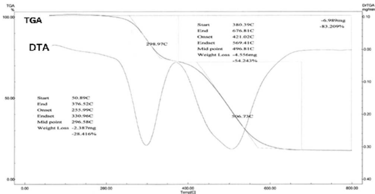
Figure 7: TGA–DTA curves of [Zn(SL 1 ) 2 ].
