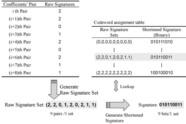
Fig. 10. Examples of signature generation.
