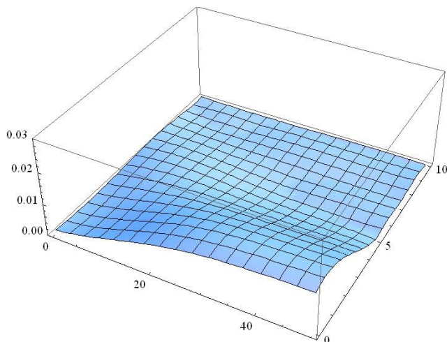
\rho(r,t) t=0 \dots 50(r_s/c) , r=0 \dots 10(r_s)
