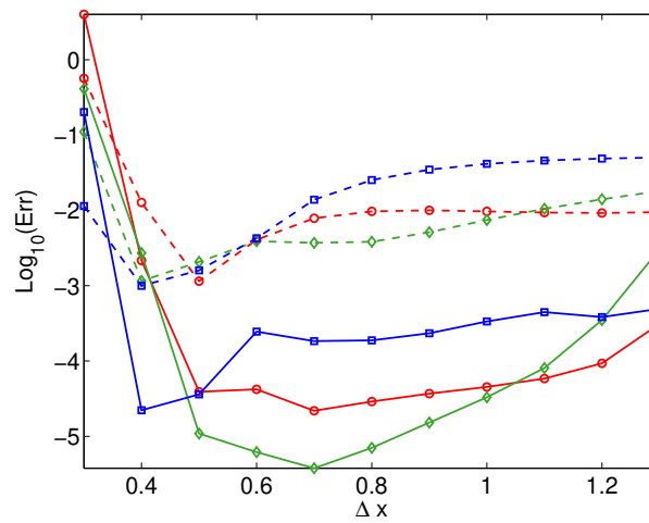
Figure 3. Logarithm of the relative error, versus grid spacing \Delta x , of the first ( \circ ), second ( \diamond ), and third ( \square ) excited state energies for the double well potential using the system-specific coherent states (—) and the harmonic oscillator coherent states (- -) with 15 basis functions.
