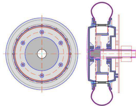
Wheel motor front and lateral views
