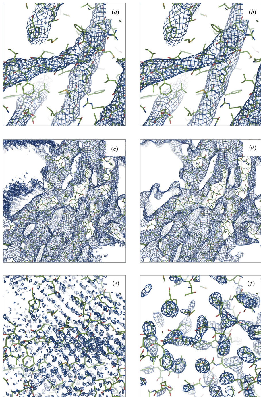
Figure 10 Maps for PDB entry 5UAR calculated by consecutive execution of the following steps: Fourier transform the original experimental map (EMDB code 8461), select a subset of Fourier coefficients of specified resolution range and finally calculate the new map using selected coefficients. Resolution ranges in Å: (a, c) 1.9–∞, (b, d) 6.7–∞, (e) 1.9–3.3, (f) 3.3–6.7. Pairs of maps (a, b) and (c, d) are the same maps shown at different contouring thresholds: high and low, respectively.
