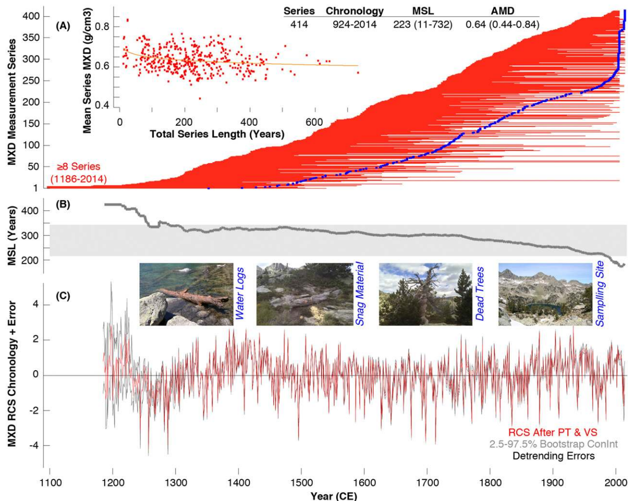
FIG. 2. (a) Distribution of 414 measurement series sorted by their first ring between 924 and 2014 (horizontal bars), whereas the blue dots refer to sample distribution when sorted by end dates. Inset reveals relationship between mean series MXD ( \text{g cm}^{-3} ) and total series length (yr), that is, higher latewood density is produced during the juvenile growth. Mean series length and average maximum latewood density (MSL and AMD) are 223 yr and 0.64 \text{ g cm}^{-3} , respectively (with minimum and maximum values ranging from 11 to 732 yr and from 0.44 to 0.84 \text{ g cm}^{-3} ). (b) Temporal evolution of the mean segment length, which is indicative of a homogeneous age structure for most of the record. (c) Examples of different data sources and site characteristics (with Lake Gerber representing the lower sampling margin), as well as the final MXD chronology between 1186 and 2014 (using RCS after power transformation and final variance stabilization) and its associated uncertainty ranges (based on bootstrap confidence intervals and composite detrending errors).
