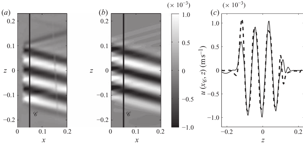
FIGURE 8. Horizontal velocity fields for (a) experiment and (b) simulation for case 12 in table 2 with M = 4 . (c) Vertical profiles along the cut \mathcal{E} located at x_\ell = 0.05 m for the experiment (---) and the simulation (—). All lengths are in metres and all velocities in metres per second.
